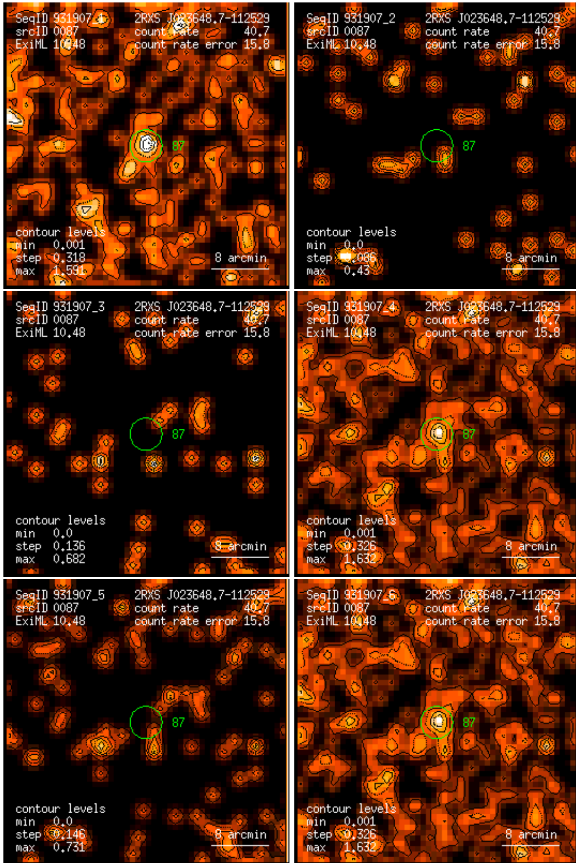
Figure 87: RASS 931907: detection 0087: band rate images, Gaussian filter: (1) PSPC channels 11 – 41, (2) 52 – 90, (3) 91 – 201, (4) 11 – 235, (5) 52 – 201, (6) 11 – 201. Broad band rates in counts/ks. Band rate contour levels in counts/ks/arcmin 2 .
