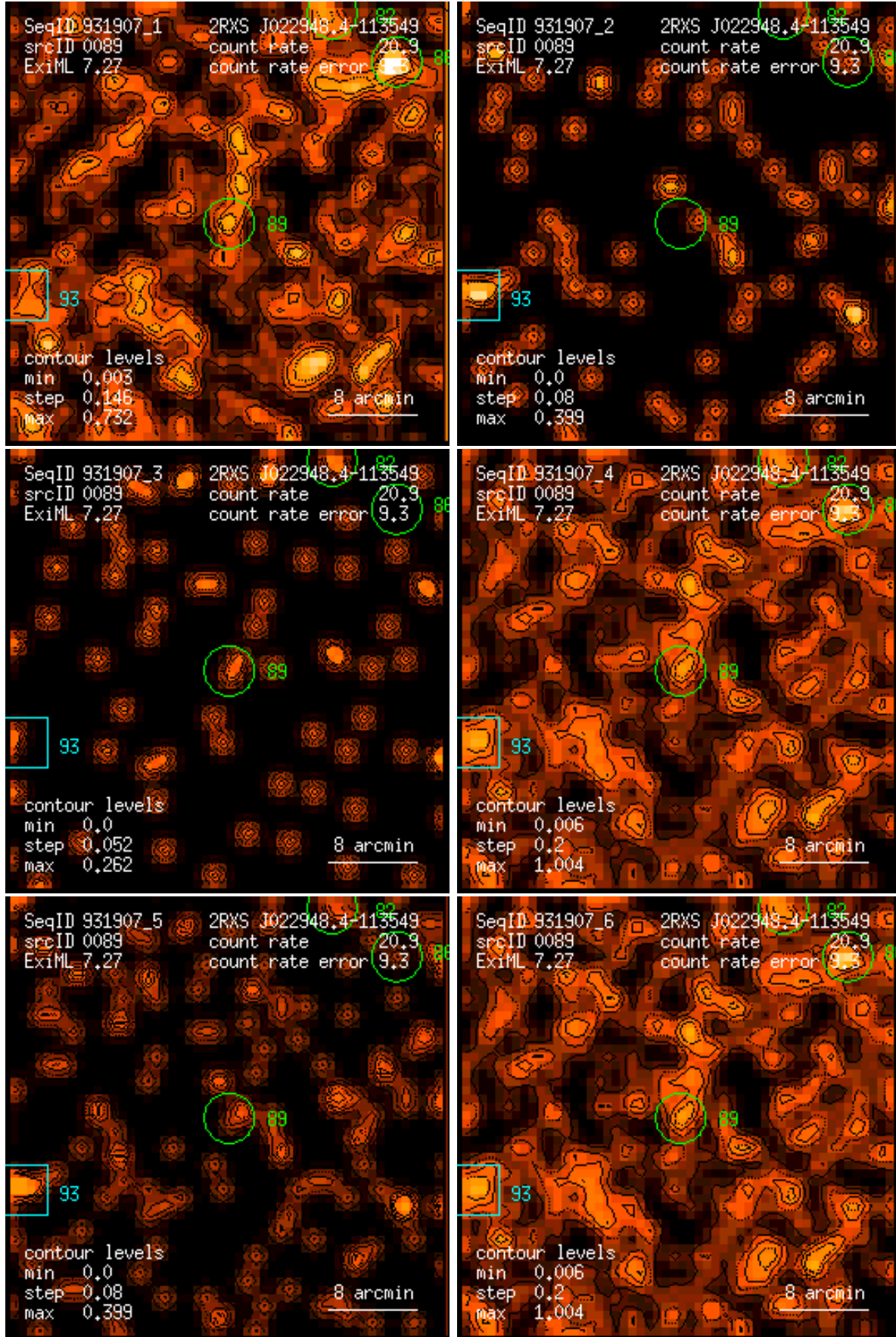
Figure 89: RASS 931907: detection 0089: band rate images, Gaussian filter: (1) PSPC channels 11 – 41, (2) 52 – 90, (3) 91 – 201, (4) 11 – 235, (5) 52 – 201, (6) 11 – 201. Broad band rates in counts/ks. Band rate contour levels in counts/ks/arcmin 2 .
