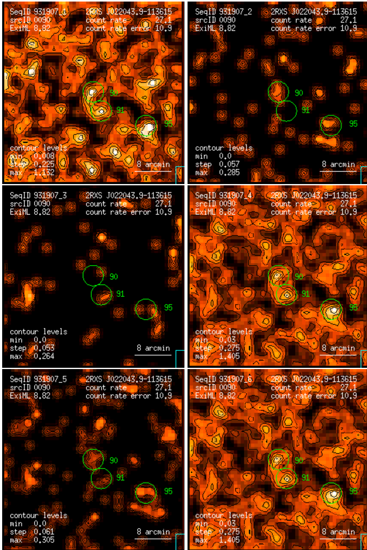
Figure 90: RASS 931907: detection 0090: band rate images, Gaussian filter: (1) PSPC channels 11 – 41, (2) 52 – 90, (3) 91 – 201, (4) 11 – 235, (5) 52 – 201, (6) 11 – 201. Broad band rates in counts/ks. Band rate contour levels in counts/ks/arcmin 2 .
