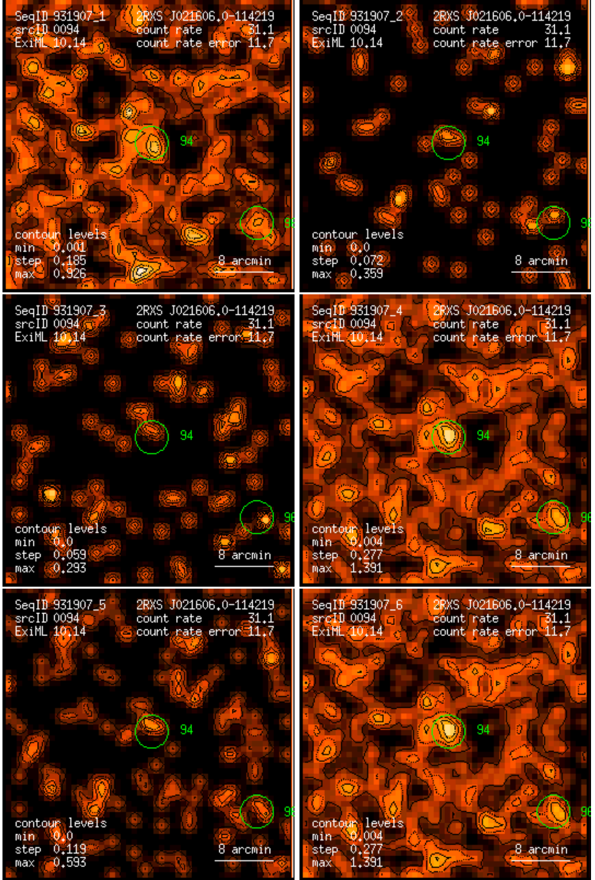
Figure 94: RASS 931907: detection 0094: band rate images, Gaussian filter: (1) PSPC channels 11 – 41, (2) 52 – 90, (3) 91 – 201, (4) 11 – 235, (5) 52 – 201, (6) 11 – 201. Broad band rates in counts/ks. Band rate contour levels in counts/ks/arcmin 2 .
