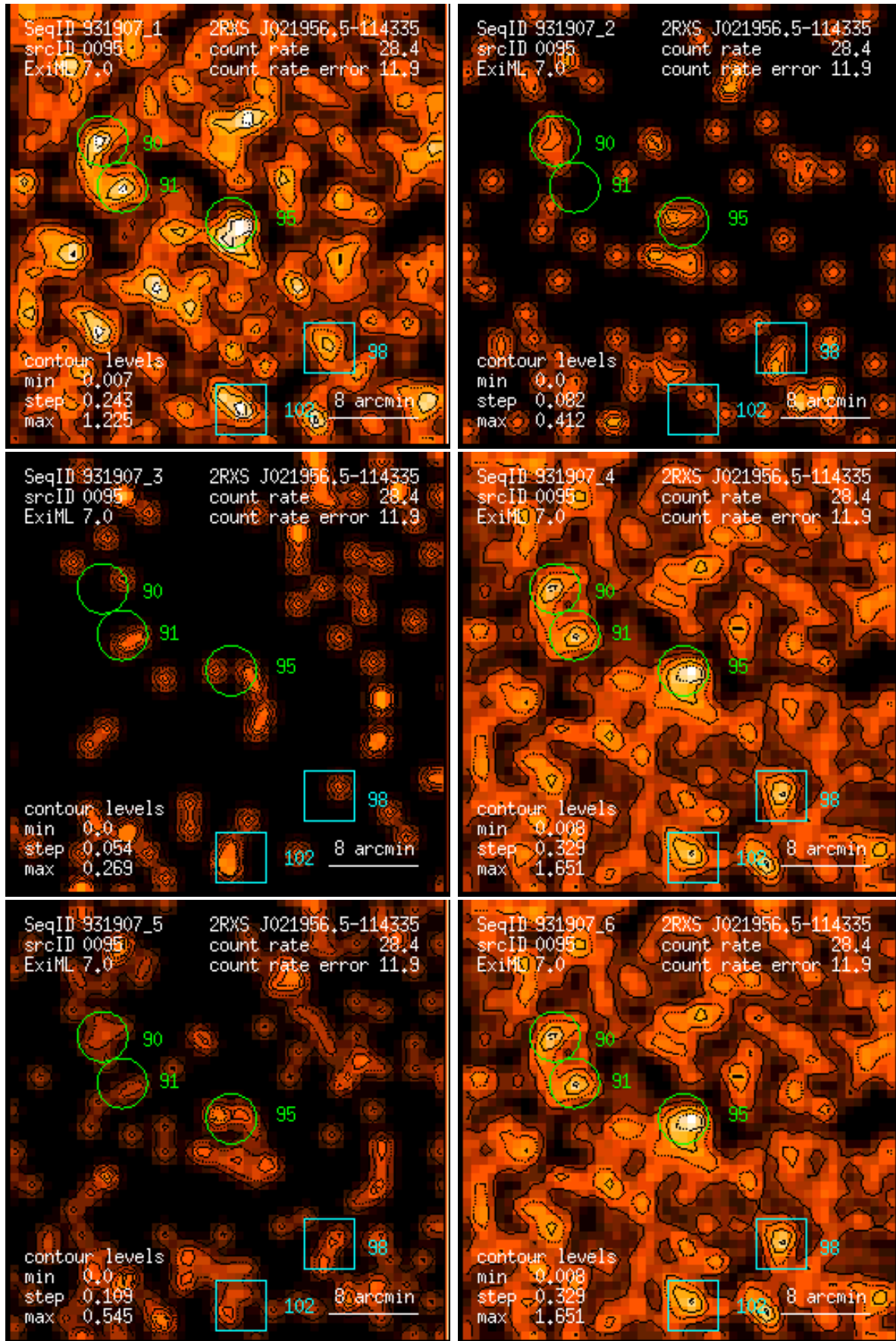
Figure 95: RASS 931907: detection 0095: band rate images, Gaussian filter: (1) PSPC channels 11 – 41, (2) 52 – 90, (3) 91 – 201, (4) 11 – 235, (5) 52 – 201, (6) 11 – 201. Broad band rates in counts/ks. Band rate contour levels in counts/ks/arcmin 2 .
