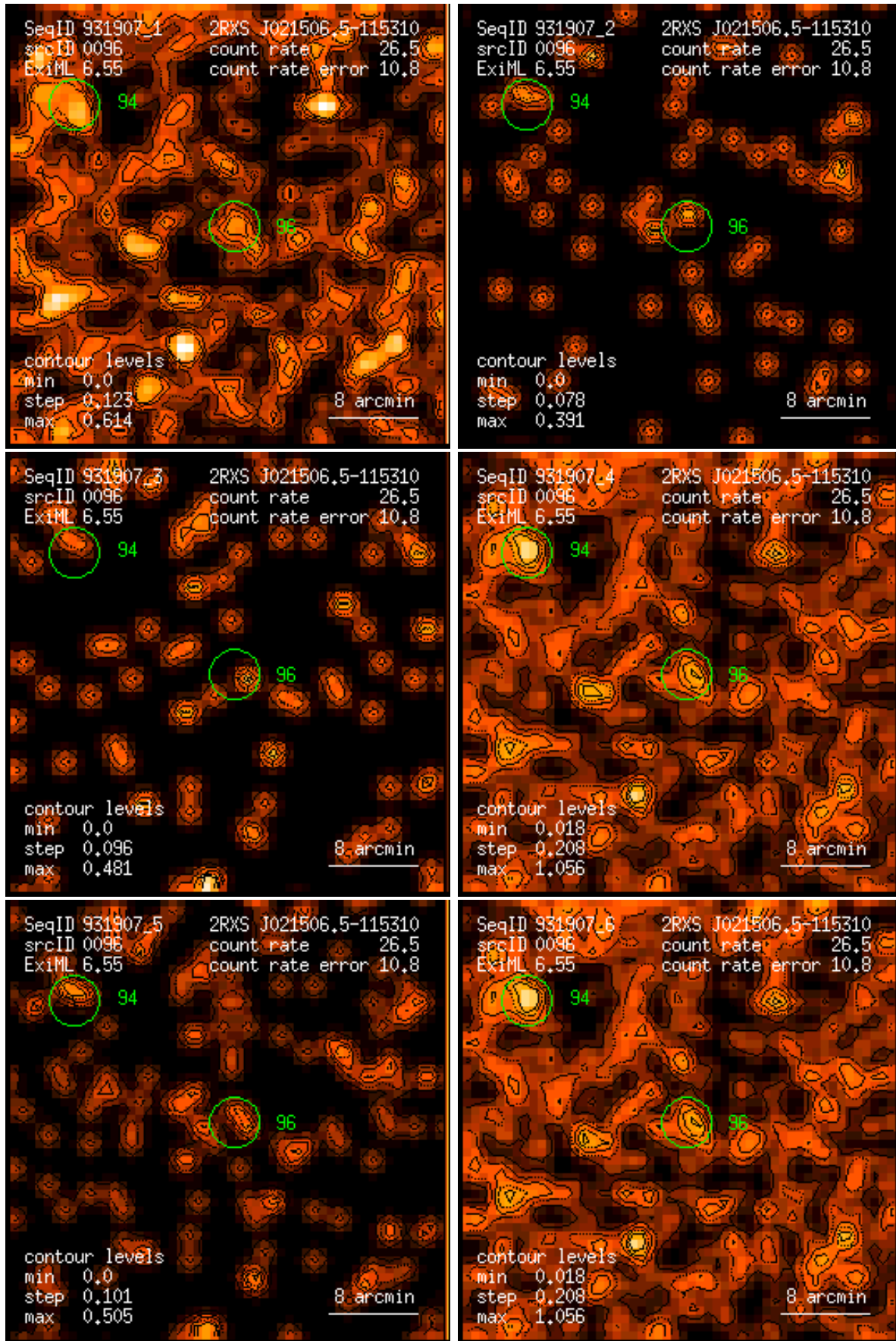
Figure 96: RASS 931907: detection 0096: band rate images, Gaussian filter: (1) PSPC channels 11 – 41, (2) 52 – 90, (3) 91 – 201, (4) 11 – 235, (5) 52 – 201, (6) 11 – 201. Broad band rates in counts/ks. Band rate contour levels in counts/ks/arcmin 2 .
