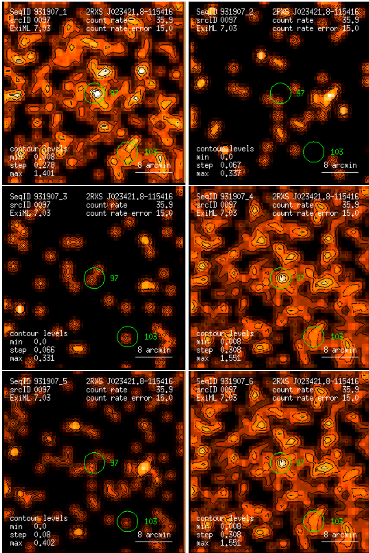
Figure 97: RASS 931907: detection 0097: band rate images, Gaussian filter: (1) PSPC channels 11 – 41, (2) 52 – 90, (3) 91 – 201, (4) 11 – 235, (5) 52 – 201, (6) 11 – 201. Broad band rates in counts/ks. Band rate contour levels in counts/ks/arcmin 2 .
