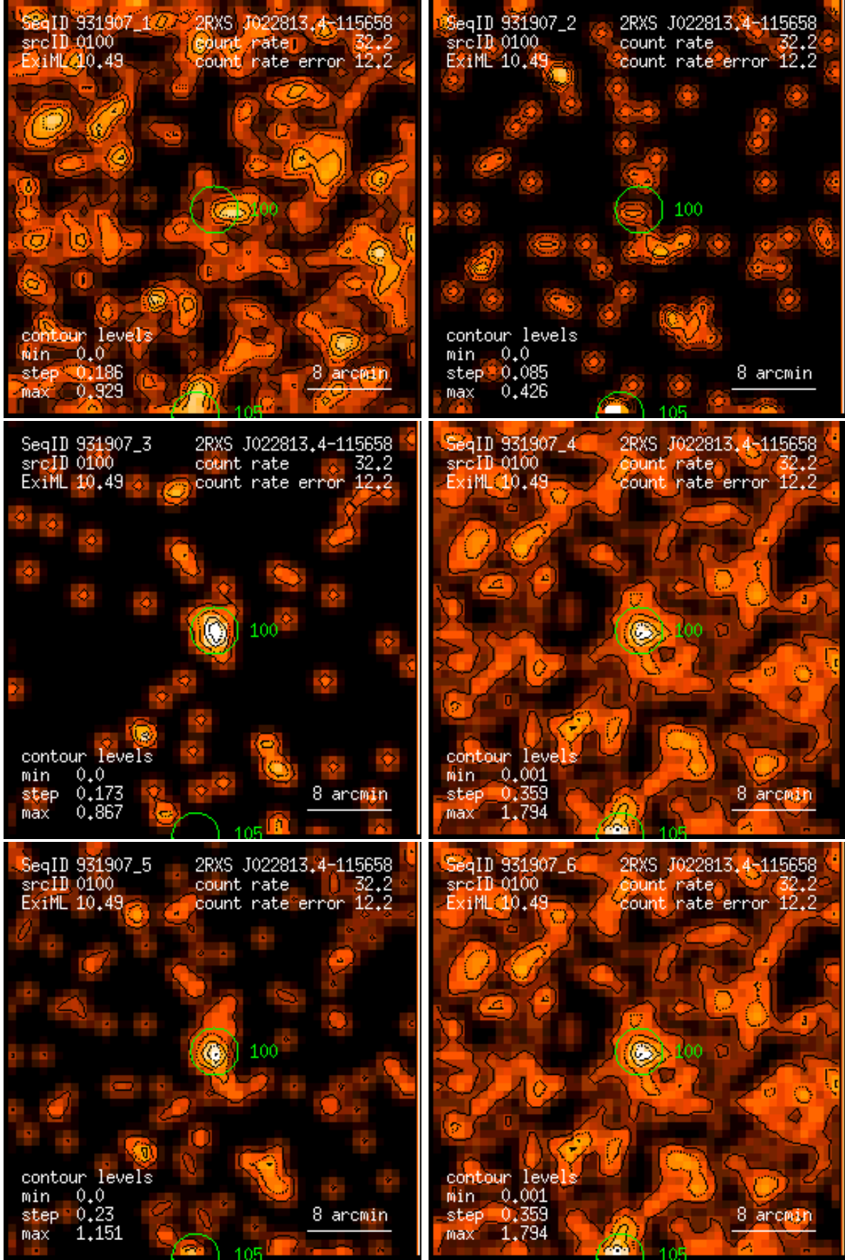
Figure 100: RASS 931907: detection 0100: band rate images, Gaussian filter: (1) PSPC channels 11 – 41, (2) 52 – 90, (3) 91 – 201, (4) 11 – 235, (5) 52 – 201, (6) 11 – 201. Broad band rates in counts/ks. Band rate contour levels in counts/ks/arcmin 2 .
