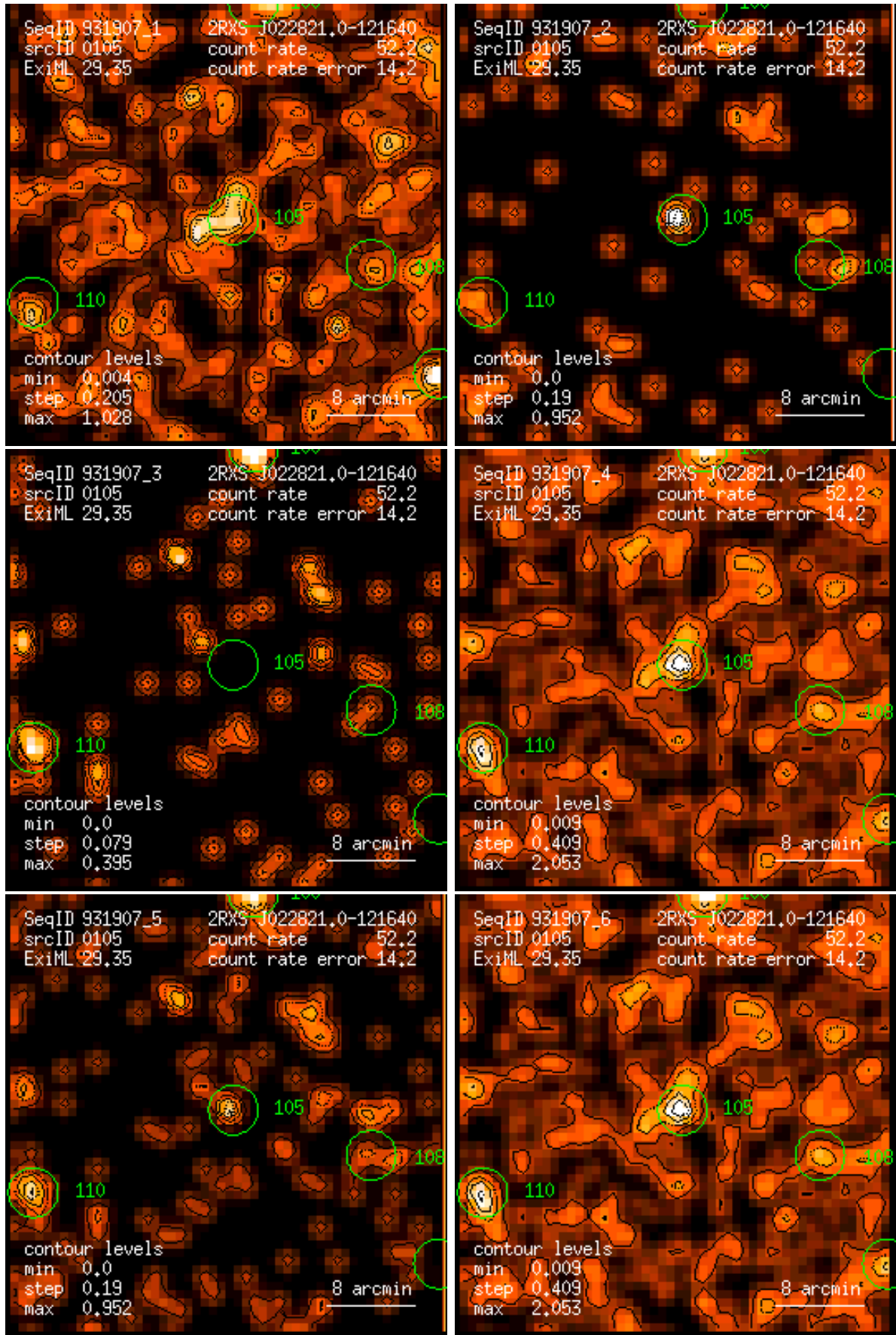
Figure 105: RASS 931907: detection 0105: band rate images, Gaussian filter: (1) PSPC channels 11 – 41, (2) 52 – 90, (3) 91 – 201, (4) 11 – 235, (5) 52 – 201, (6) 11 – 201. Broad band rates in counts/ks. Band rate contour levels in counts/ks/arcmin 2 .
