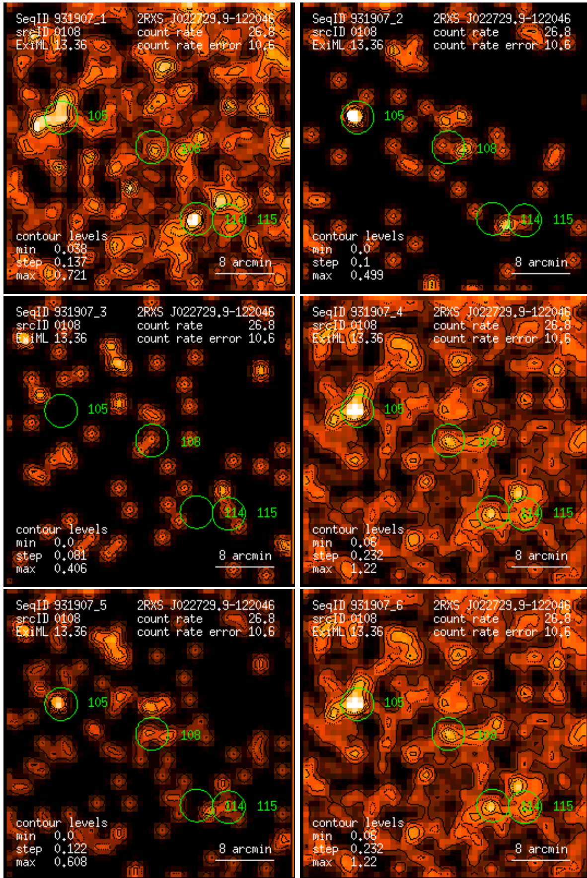
Figure 108: RASS 931907: detection 0108: band rate images, Gaussian filter: (1) PSPC channels 11 – 41, (2) 52 – 90, (3) 91 – 201, (4) 11 – 235, (5) 52 – 201, (6) 11 – 201. Broad band rates in counts/ks. Band rate contour levels in counts/ks/arcmin 2 .
