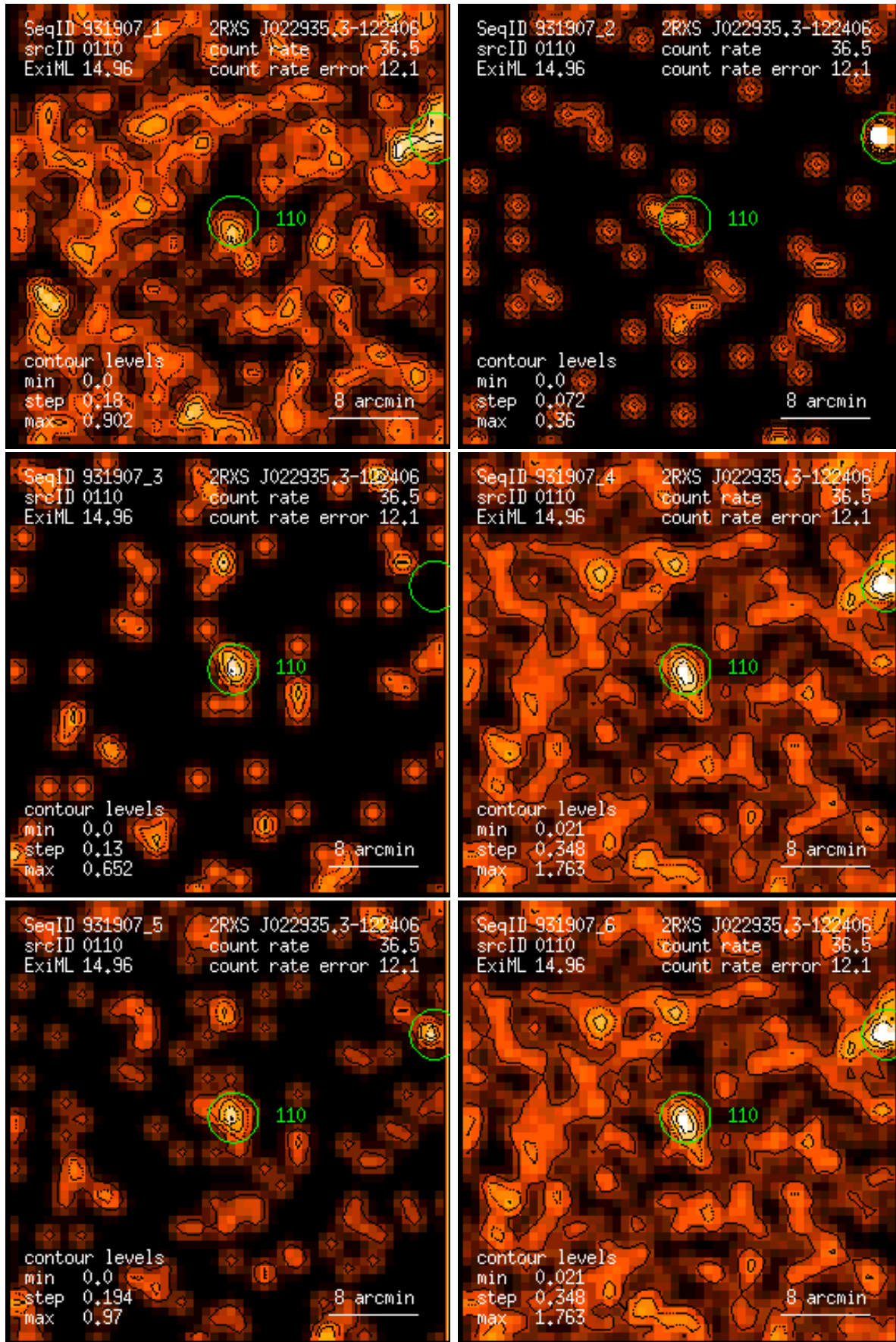
Figure 110: RASS 931907: detection 0110: band rate images, Gaussian filter: (1) PSPC channels 11 – 41, (2) 52 – 90, (3) 91 – 201, (4) 11 – 235, (5) 52 – 201, (6) 11 – 201. Broad band rates in counts/ks. Band rate contour levels in counts/ks/arcmin 2 .
