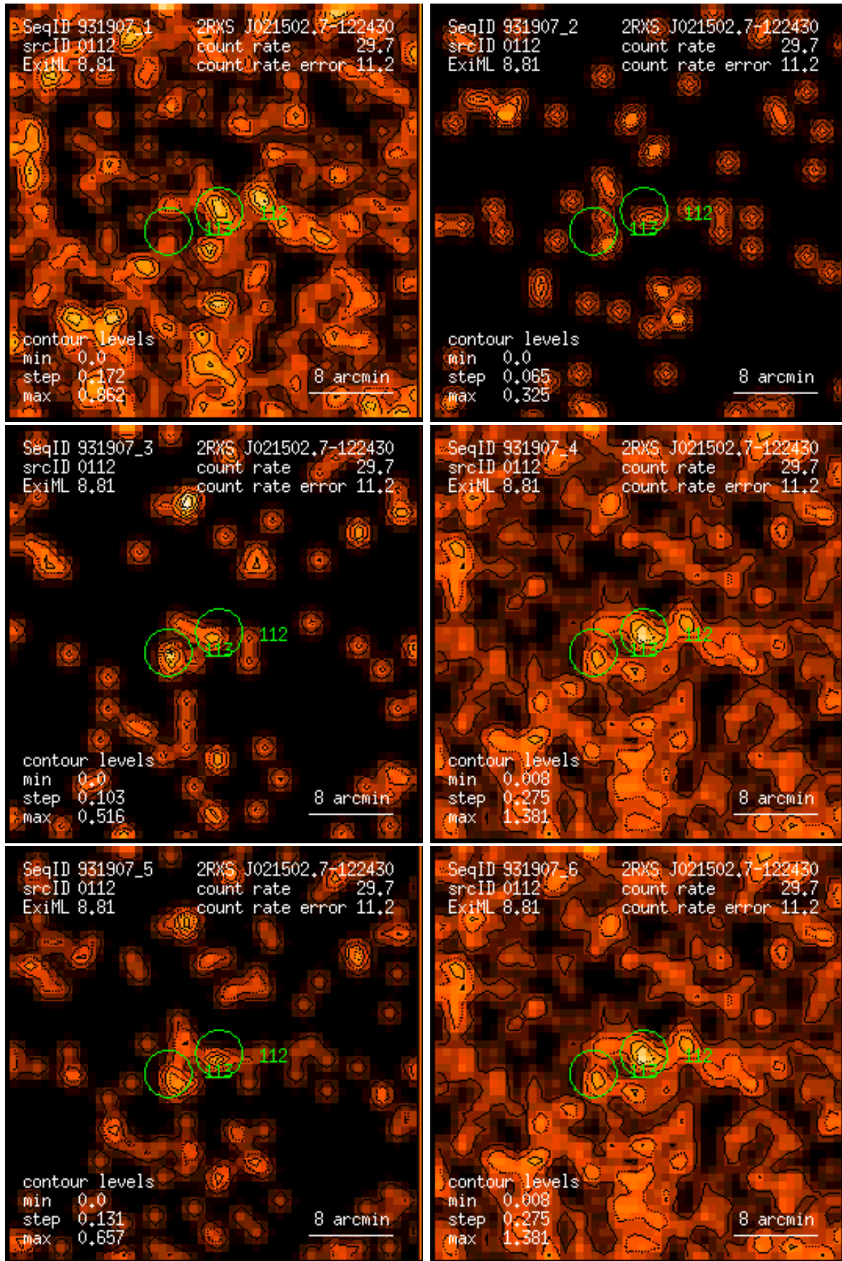
Figure 112: RASS 931907: detection 0112: band rate images, Gaussian filter: (1) PSPC channels 11 – 41, (2) 52 – 90, (3) 91 – 201, (4) 11 – 235, (5) 52 – 201, (6) 11 – 201. Broad band rates in counts/ks. Band rate contour levels in counts/ks/arcmin 2 .
