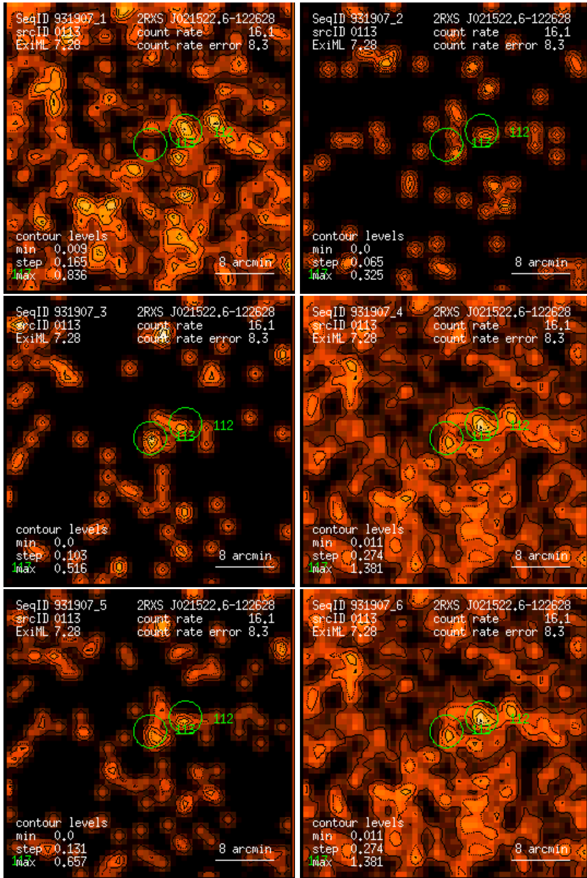
Figure 113: RASS 931907: detection 0113: band rate images, Gaussian filter: (1) PSPC channels 11 – 41, (2) 52 – 90, (3) 91 – 201, (4) 11 – 235, (5) 52 – 201, (6) 11 – 201. Broad band rates in counts/ks. Band rate contour levels in counts/ks/arcmin 2 .
