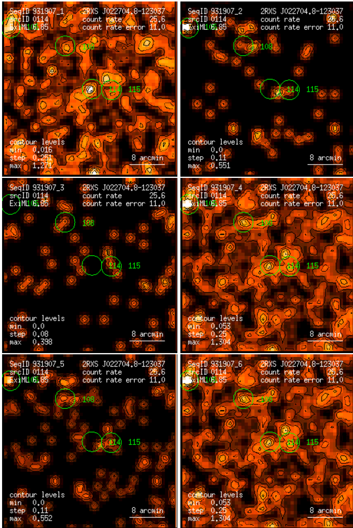
Figure 114: RASS 931907: detection 0114: band rate images, Gaussian filter: (1) PSPC channels 11 – 41, (2) 52 – 90, (3) 91 – 201, (4) 11 – 235, (5) 52 – 201, (6) 11 – 201. Broad band rates in counts/ks. Band rate contour levels in counts/ks/arcmin 2 .
