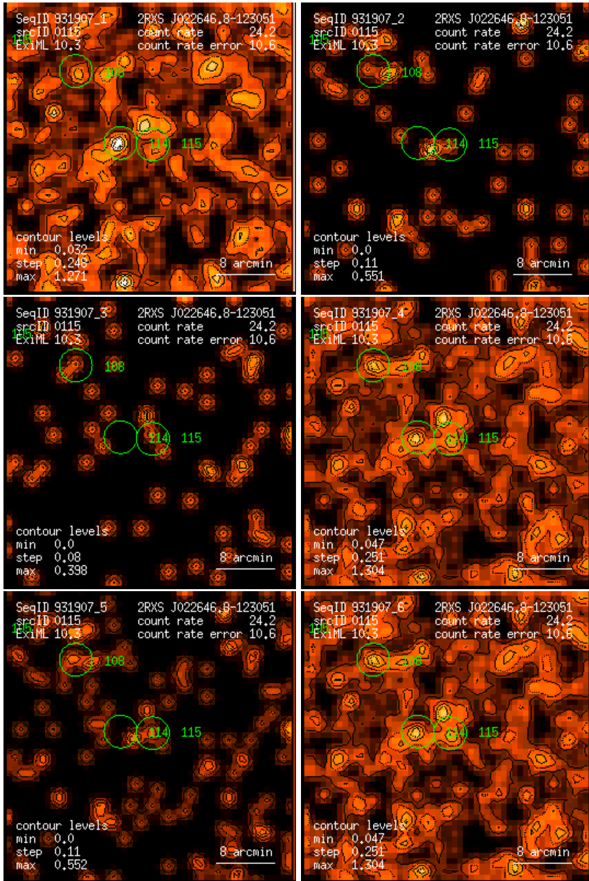
Figure 115: RASS 931907: detection 0115: band rate images, Gaussian filter: (1) PSPC channels 11 – 41, (2) 52 – 90, (3) 91 – 201, (4) 11 – 235, (5) 52 – 201, (6) 11 – 201. Broad band rates in counts/ks. Band rate contour levels in counts/ks/arcmin 2 .
