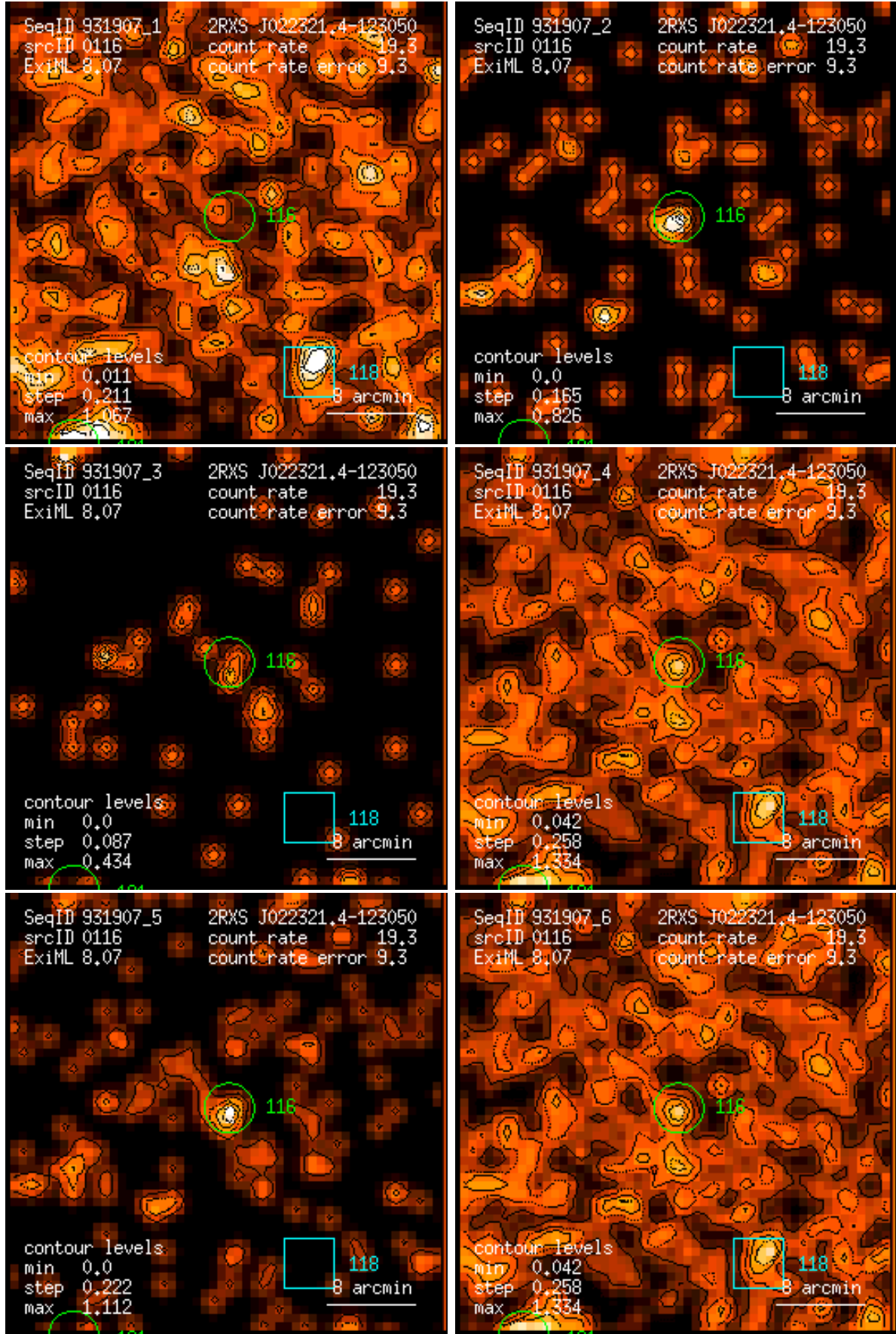
Figure 116: RASS 931907: detection 0116: band rate images, Gaussian filter: (1) PSPC channels 11 – 41, (2) 52 – 90, (3) 91 – 201, (4) 11 – 235, (5) 52 – 201, (6) 11 – 201. Broad band rates in counts/ks. Band rate contour levels in counts/ks/arcmin 2 .
