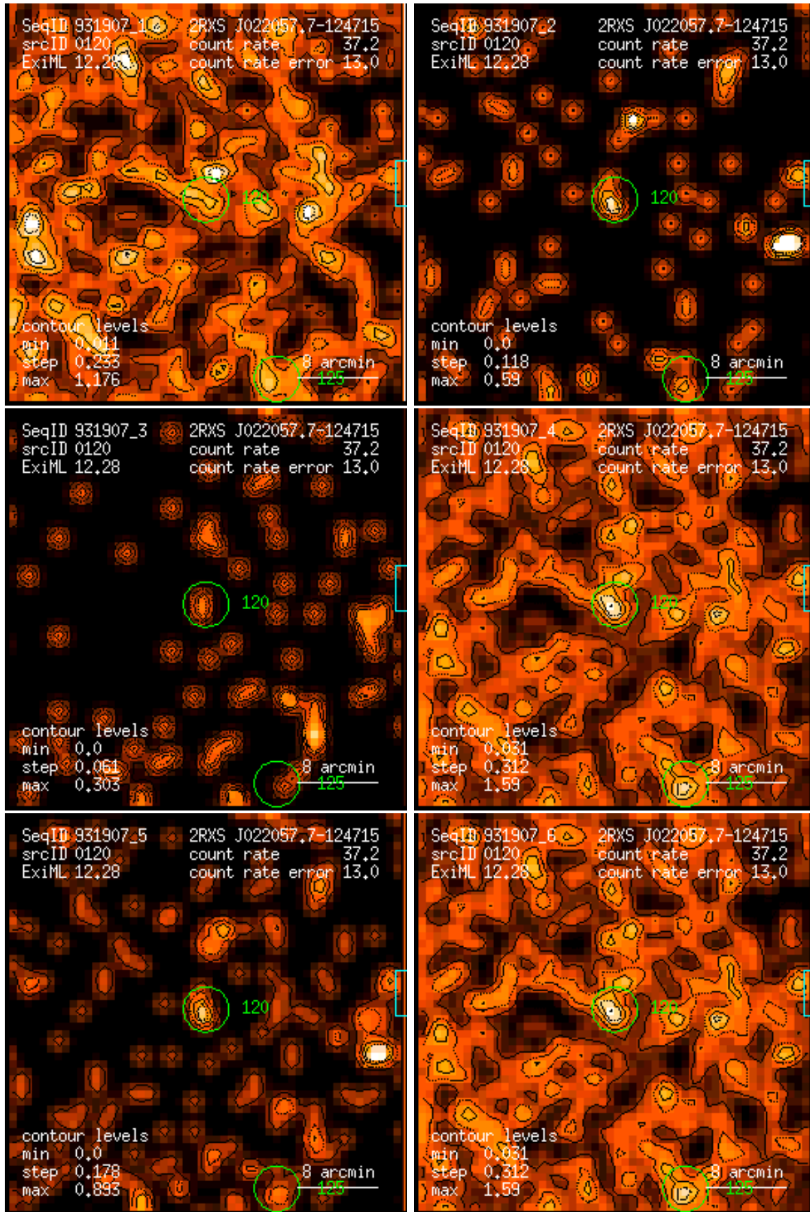
Figure 120: RASS 931907: detection 0120: band rate images, Gaussian filter: (1) PSPC channels 11 – 41, (2) 52 – 90, (3) 91 – 201, (4) 11 – 235, (5) 52 – 201, (6) 11 – 201. Broad band rates in counts/ks. Band rate contour levels in counts/ks/arcmin 2 .
