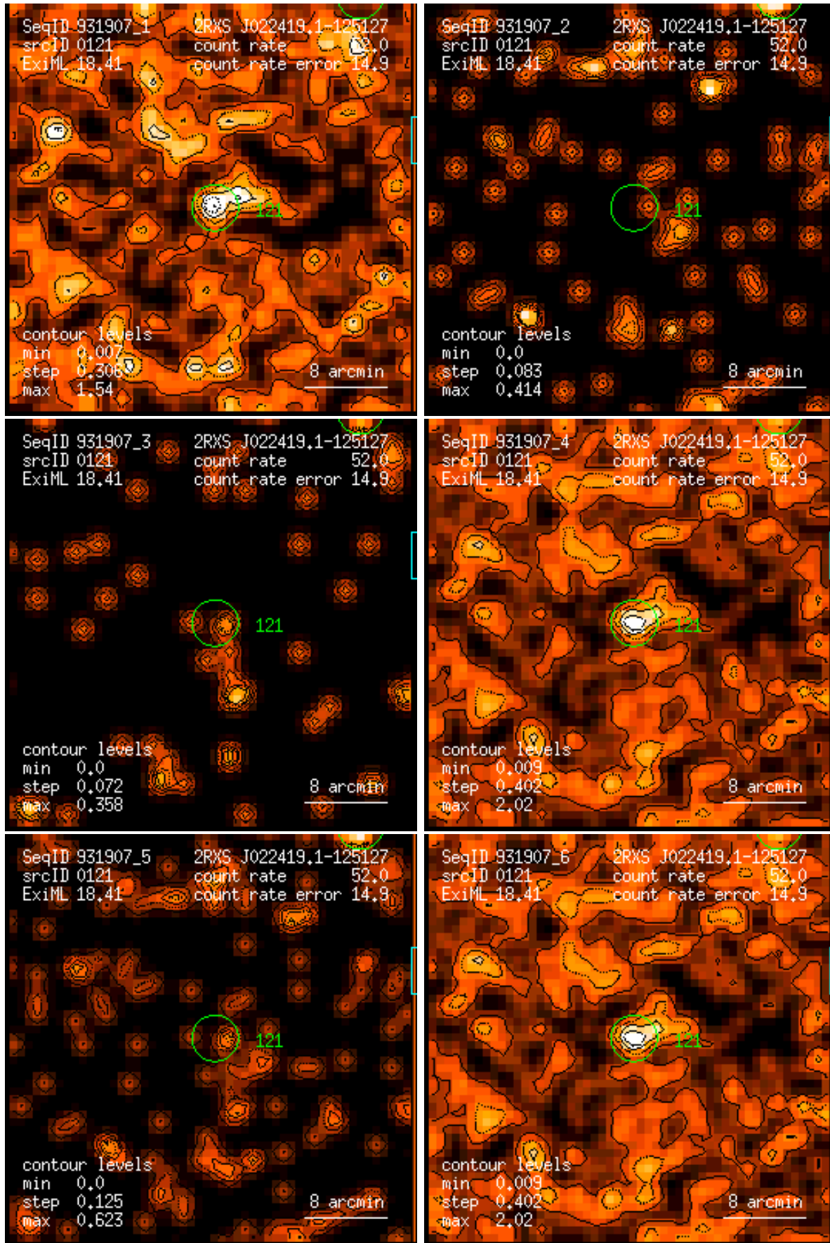
Figure 121: RASS 931907: detection 0121: band rate images, Gaussian filter: (1) PSPC channels 11 – 41, (2) 52 – 90, (3) 91 – 201, (4) 11 – 235, (5) 52 – 201, (6) 11 – 201. Broad band rates in counts/ks. Band rate contour levels in counts/ks/arcmin 2 .
