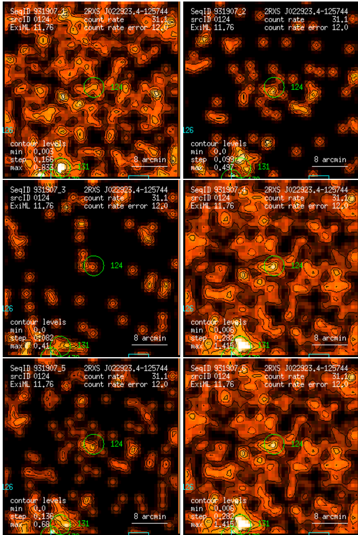
Figure 124: RASS 931907: detection 0124: band rate images, Gaussian filter: (1) PSPC channels 11 – 41, (2) 52 – 90, (3) 91 – 201, (4) 11 – 235, (5) 52 – 201, (6) 11 – 201. Broad band rates in counts/ks. Band rate contour levels in counts/ks/arcmin 2 .
