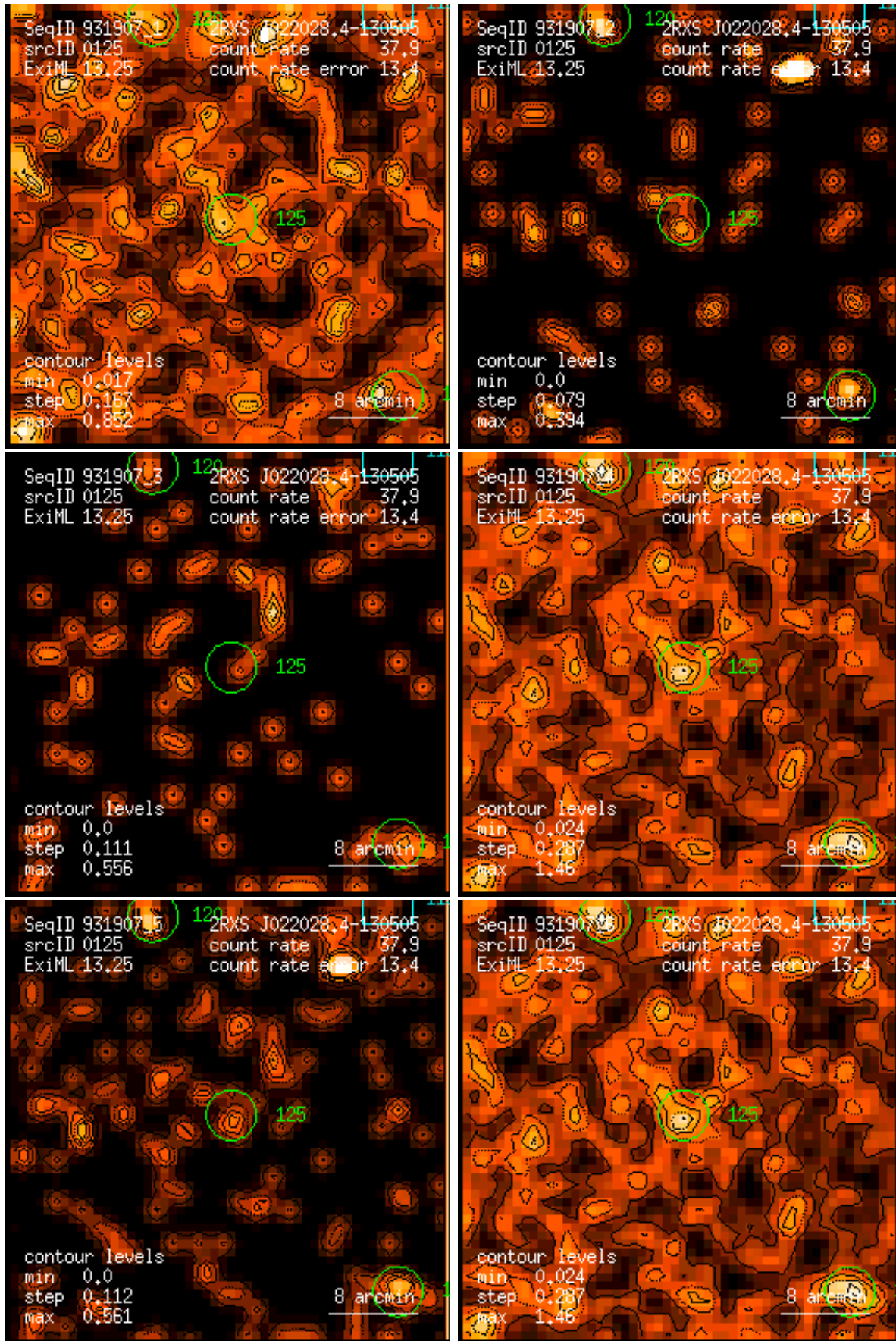
Figure 125: RASS 931907: detection 0125: band rate images, Gaussian filter: (1) PSPC channels 11 – 41, (2) 52 – 90, (3) 91 – 201, (4) 11 – 235, (5) 52 – 201, (6) 11 – 201. Broad band rates in counts/ks. Band rate contour levels in counts/ks/arcmin 2 .
