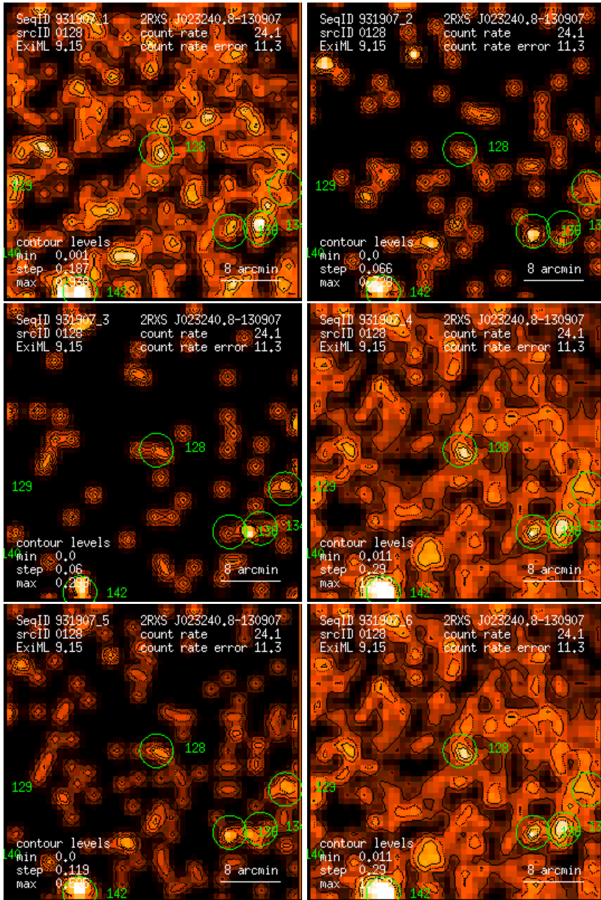
Figure 128: RASS 931907: detection 0128: band rate images, Gaussian filter: (1) PSPC channels 11 – 41, (2) 52 – 90, (3) 91 – 201, (4) 11 – 235, (5) 52 – 201, (6) 11 – 201. Broad band rates in counts/ks. Band rate contour levels in counts/ks/arcmin 2 .
