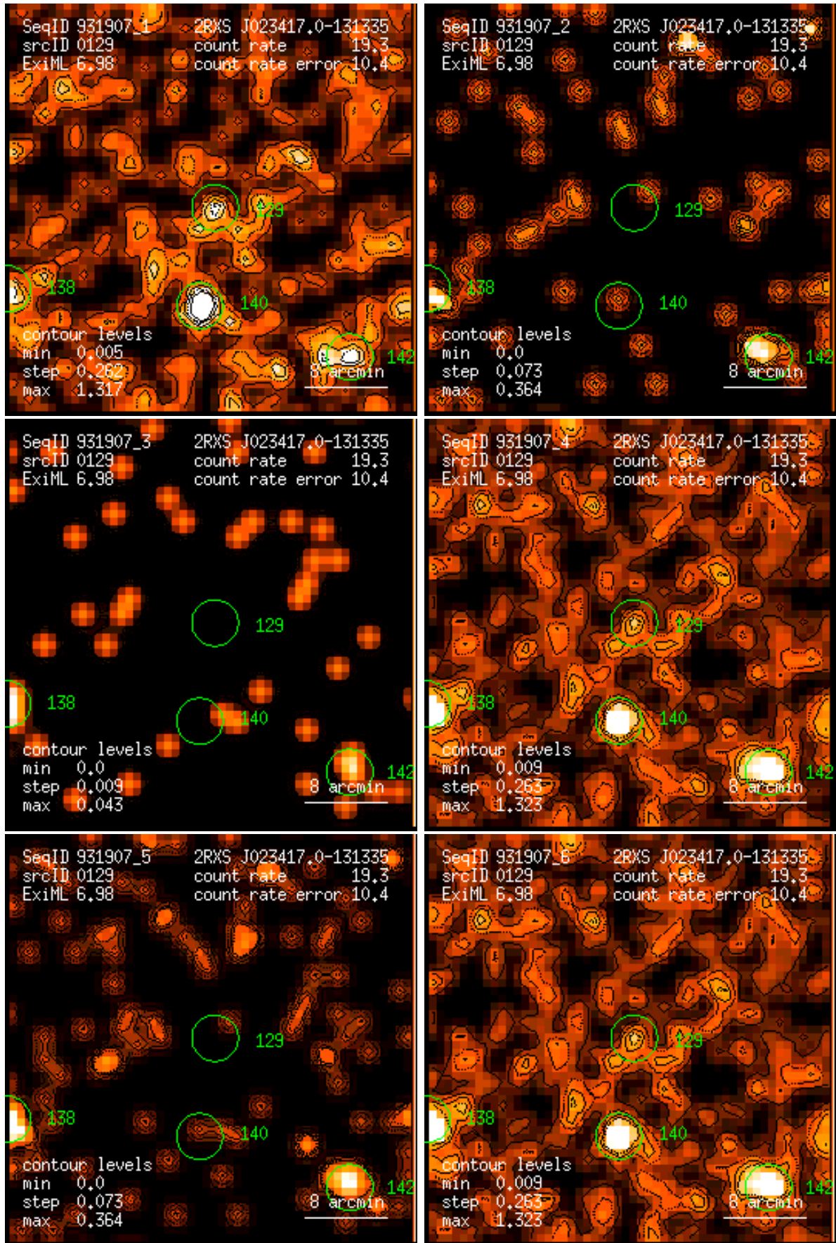
Figure 129: RASS 931907: detection 0129: band rate images, Gaussian filter: (1) PSPC channels 11 – 41, (2) 52 – 90, (3) 91 – 201, (4) 11 – 235, (5) 52 – 201, (6) 11 – 201. Broad band rates in counts/ks. Band rate contour levels in counts/ks/arcmin 2 .
