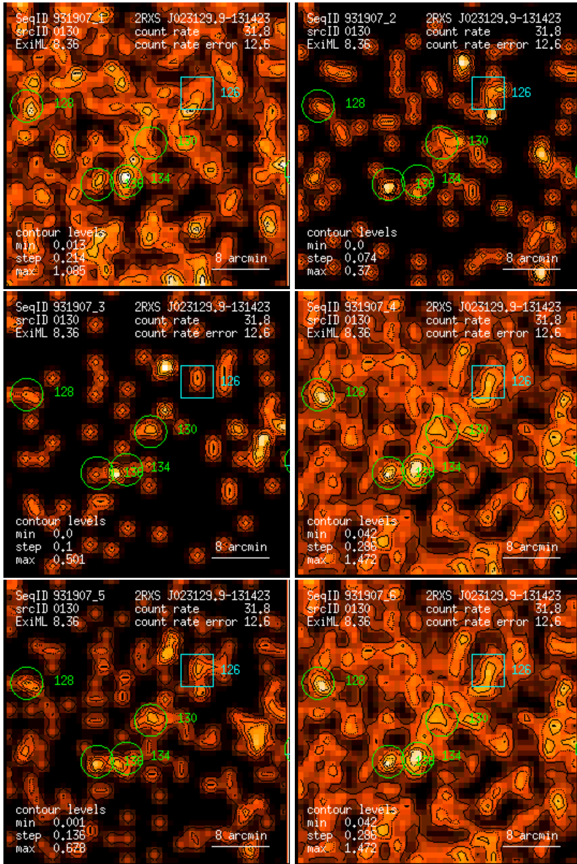
Figure 130: RASS 931907: detection 0130: band rate images, Gaussian filter: (1) PSPC channels 11 – 41, (2) 52 – 90, (3) 91 – 201, (4) 11 – 235, (5) 52 – 201, (6) 11 – 201. Broad band rates in counts/ks. Band rate contour levels in counts/ks/arcmin 2 .
