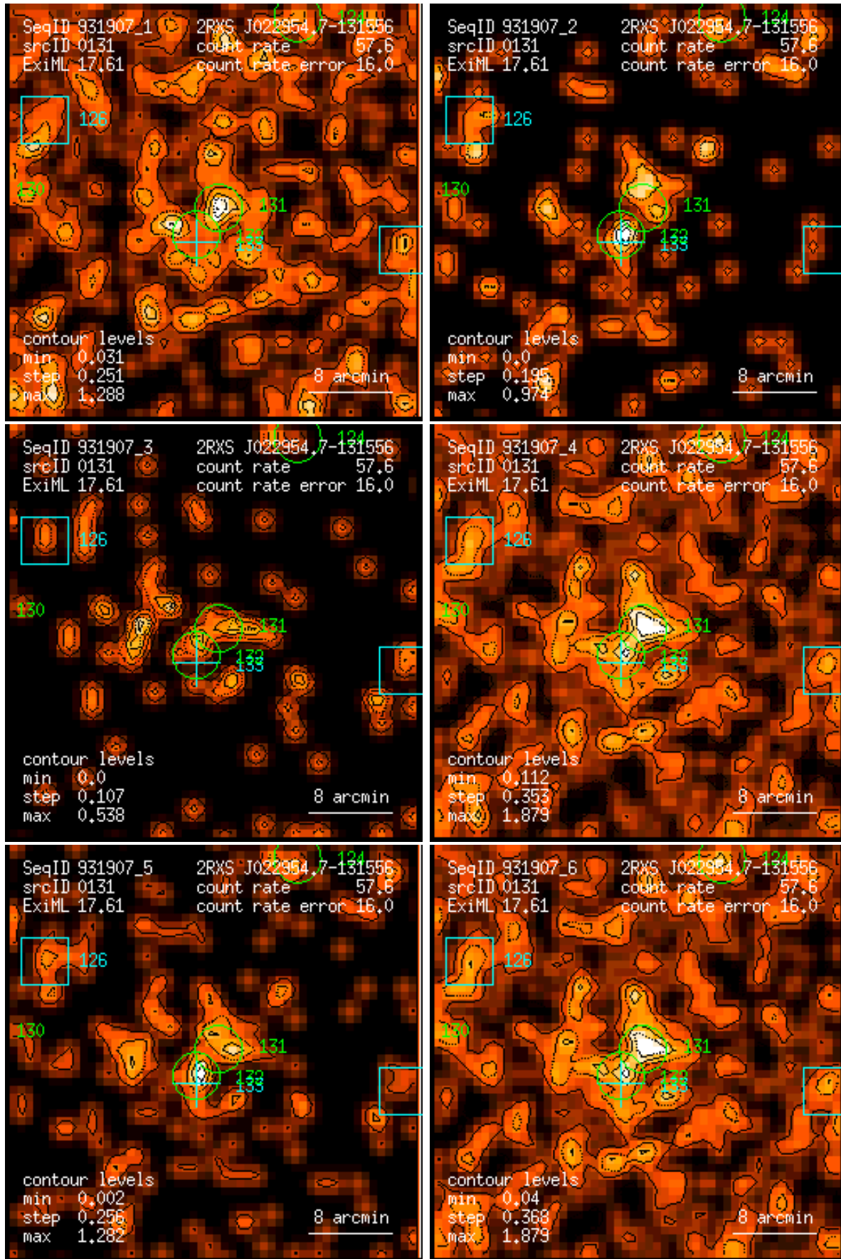
Figure 131: RASS 931907: detection 0131: band rate images, Gaussian filter: (1) PSPC channels 11 – 41, (2) 52 – 90, (3) 91 – 201, (4) 11 – 235, (5) 52 – 201, (6) 11 – 201. Broad band rates in counts/ks. Band rate contour levels in counts/ks/arcmin 2 .
