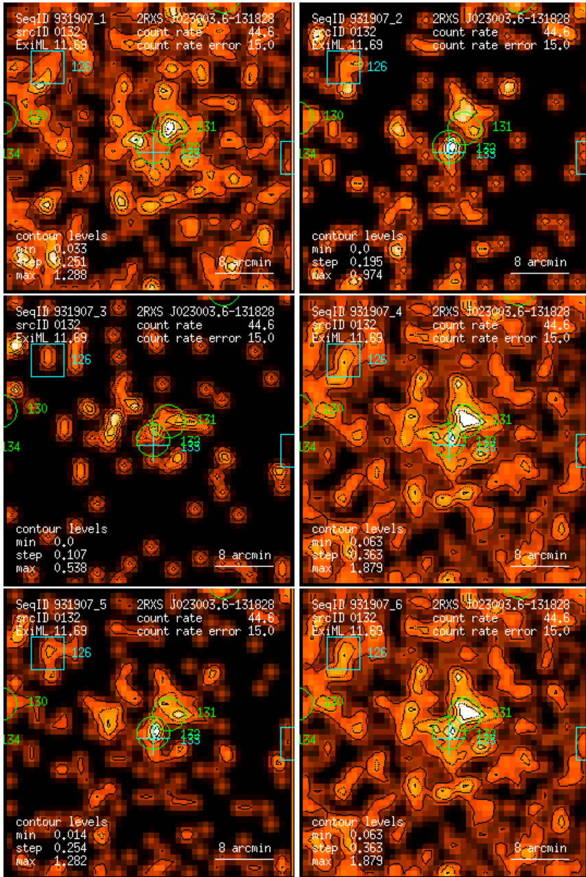
Figure 132: RASS 931907: detection 0132: band rate images, Gaussian filter: (1) PSPC channels 11 – 41, (2) 52 – 90, (3) 91 – 201, (4) 11 – 235, (5) 52 – 201, (6) 11 – 201. Broad band rates in counts/ks. Band rate contour levels in counts/ks/arcmin 2 .
