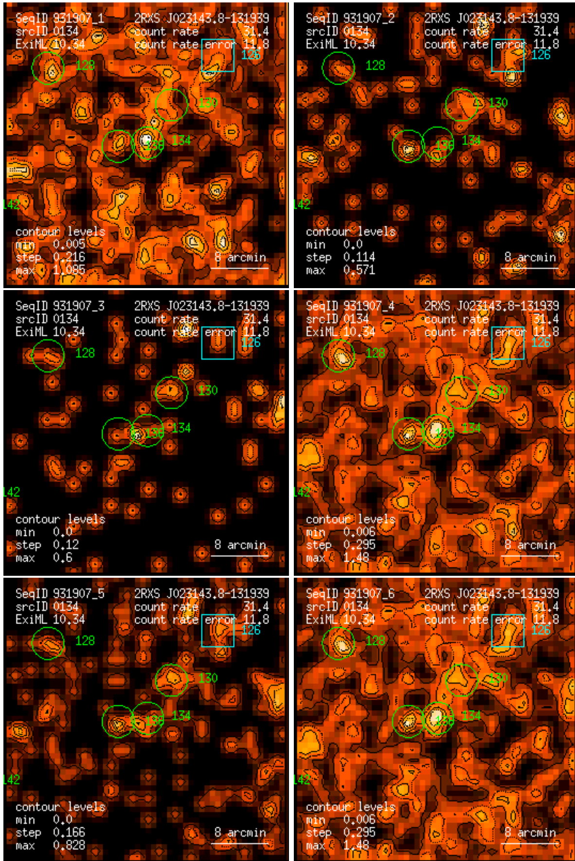
Figure 134: RASS 931907: detection 0134: band rate images, Gaussian filter: (1) PSPC channels 11 – 41, (2) 52 – 90, (3) 91 – 201, (4) 11 – 235, (5) 52 – 201, (6) 11 – 201. Broad band rates in counts/ks. Band rate contour levels in counts/ks/arcmin 2 .
