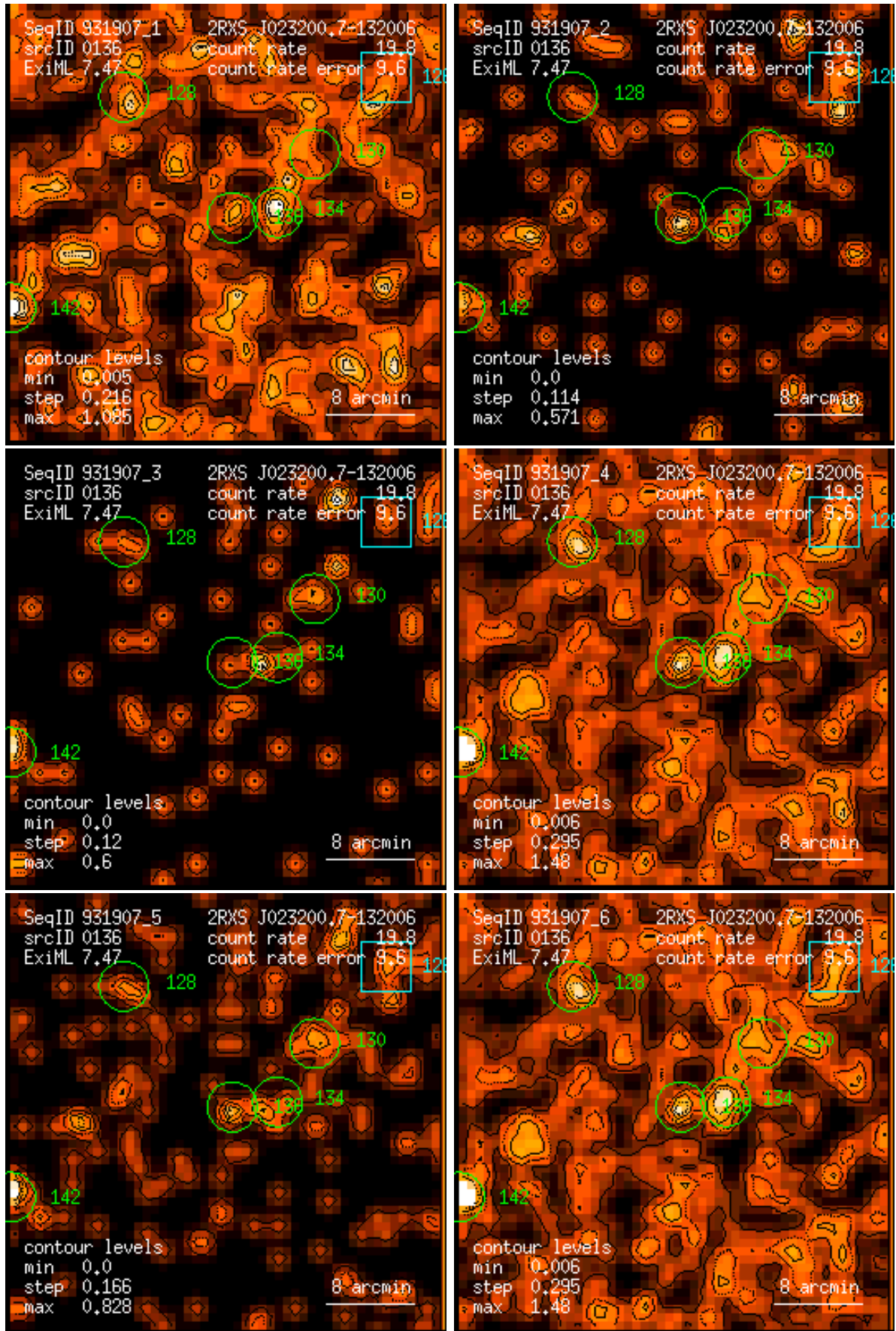
Figure 136: RASS 931907: detection 0136: band rate images, Gaussian filter: (1) PSPC channels 11 – 41, (2) 52 – 90, (3) 91 – 201, (4) 11 – 235, (5) 52 – 201, (6) 11 – 201. Broad band rates in counts/ks. Band rate contour levels in counts/ks/arcmin 2 .
