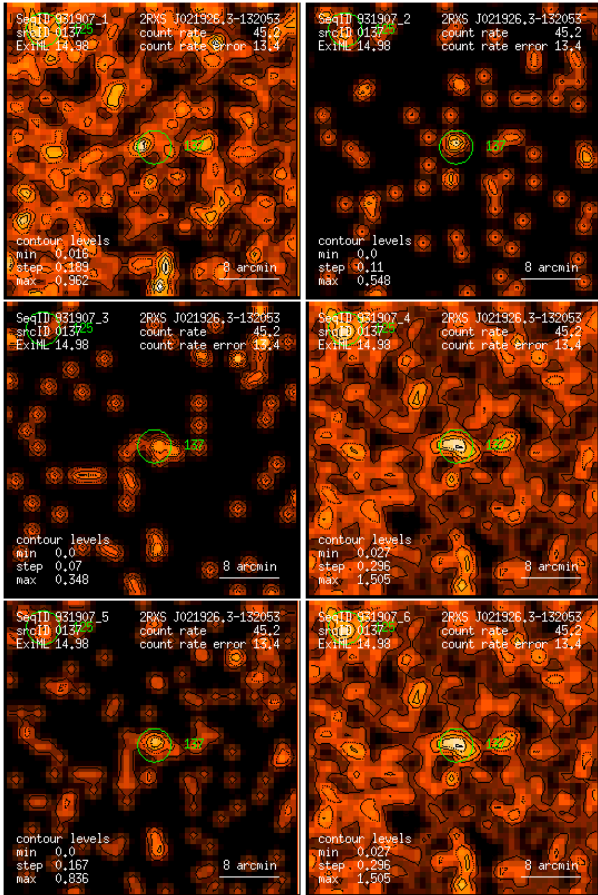
Figure 137: RASS 931907: detection 0137: band rate images, Gaussian filter: (1) PSPC channels 11 – 41, (2) 52 – 90, (3) 91 – 201, (4) 11 – 235, (5) 52 – 201, (6) 11 – 201. Broad band rates in counts/ks. Band rate contour levels in counts/ks/arcmin 2 .
