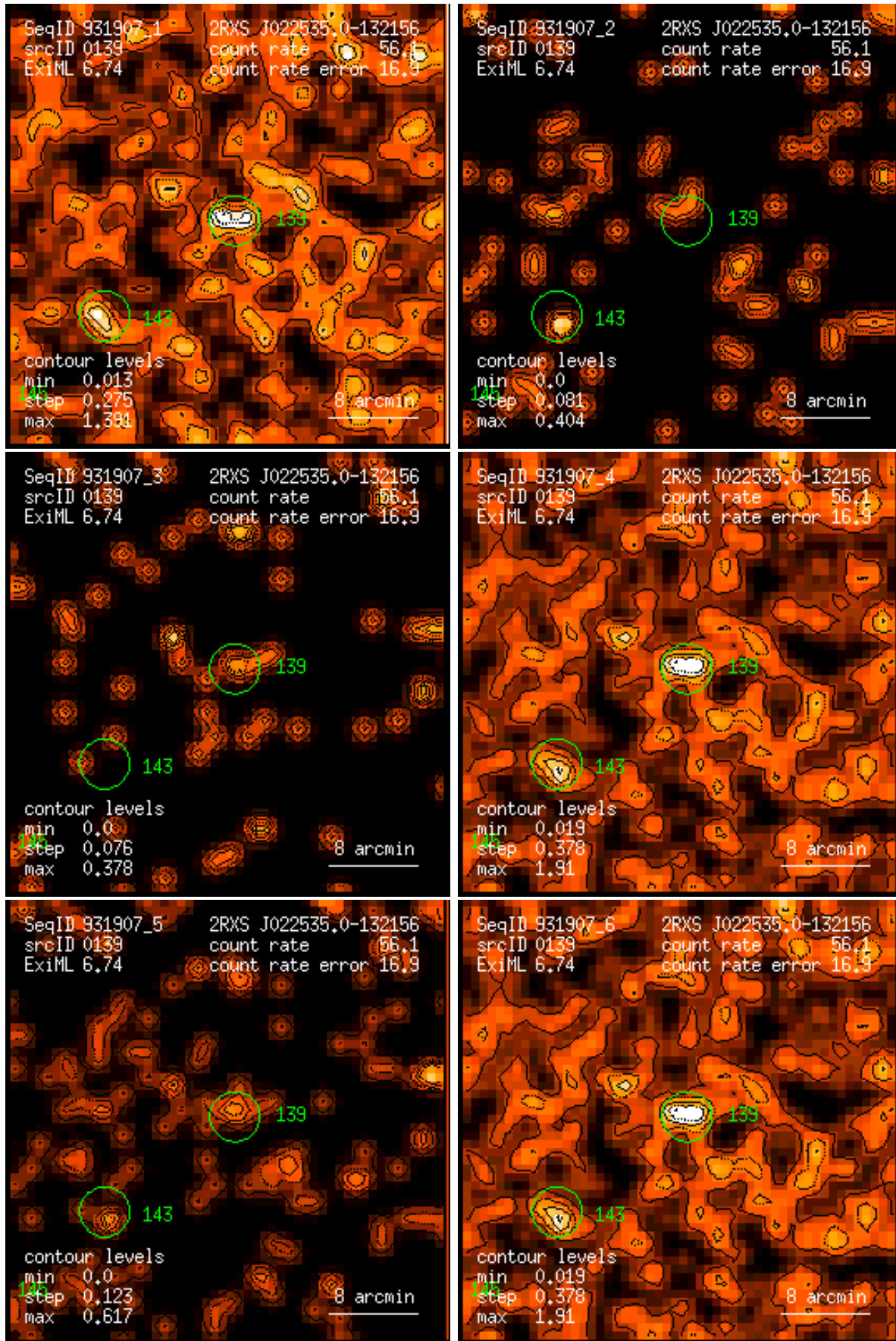
Figure 139: RASS 931907: detection 0139: band rate images, Gaussian filter: (1) PSPC channels 11 – 41, (2) 52 – 90, (3) 91 – 201, (4) 11 – 235, (5) 52 – 201, (6) 11 – 201. Broad band rates in counts/ks. Band rate contour levels in counts/ks/arcmin 2 .
