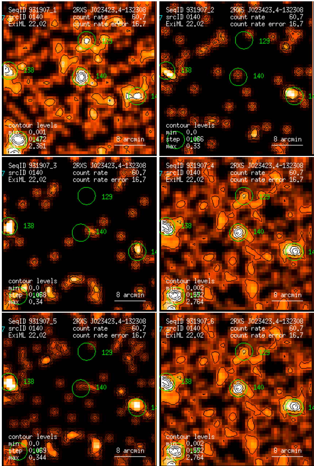
Figure 140: RASS 931907: detection 0140: band rate images, Gaussian filter: (1) PSPC channels 11 – 41, (2) 52 – 90, (3) 91 – 201, (4) 11 – 235, (5) 52 – 201, (6) 11 – 201. Broad band rates in counts/ks. Band rate contour levels in counts/ks/arcmin 2 .
