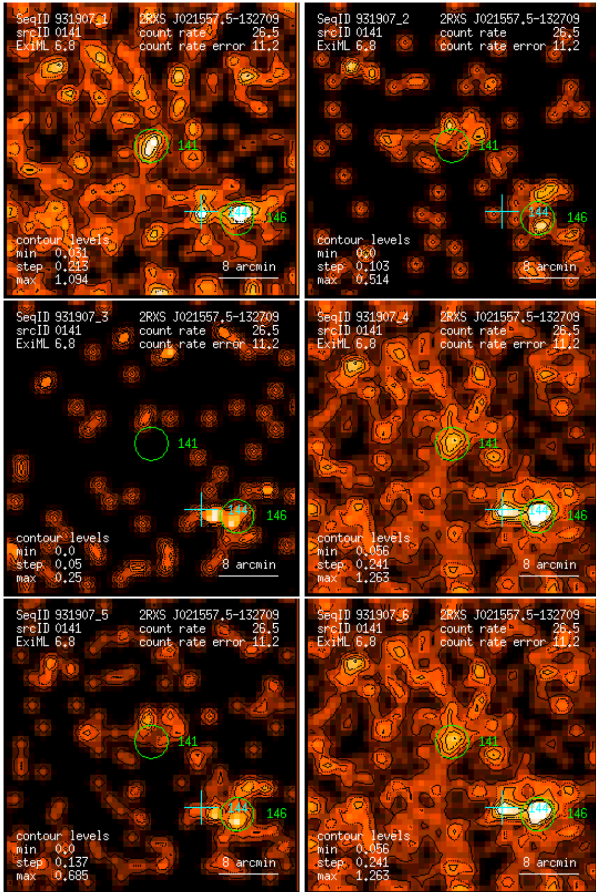
Figure 141: RASS 931907: detection 0141: band rate images, Gaussian filter: (1) PSPC channels 11 – 41, (2) 52 – 90, (3) 91 – 201, (4) 11 – 235, (5) 52 – 201, (6) 11 – 201. Broad band rates in counts/ks. Band rate contour levels in counts/ks/arcmin 2 .
