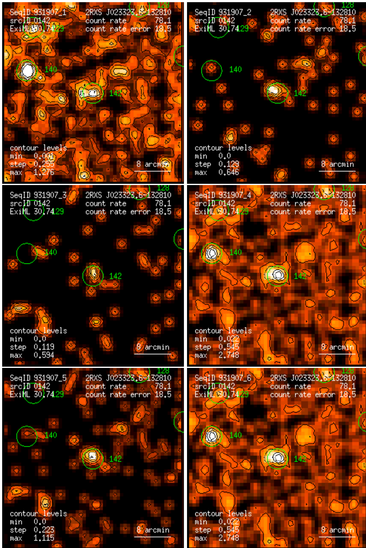
Figure 142: RASS 931907: detection 0142: band rate images, Gaussian filter: (1) PSPC channels 11 – 41, (2) 52 – 90, (3) 91 – 201, (4) 11 – 235, (5) 52 – 201, (6) 11 – 201. Broad band rates in counts/ks. Band rate contour levels in counts/ks/arcmin 2 .
