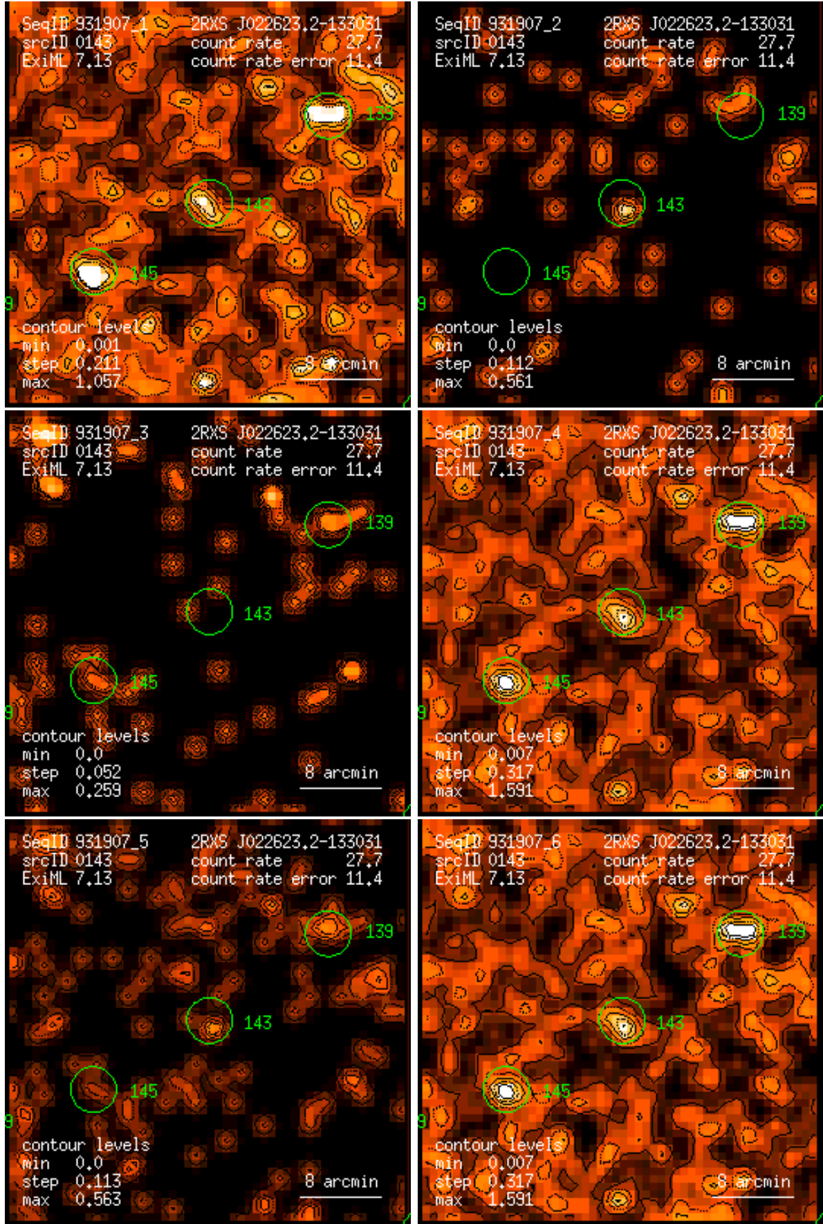
Figure 143: RASS 931907: detection 0143: band rate images, Gaussian filter: (1) PSPC channels 11 – 41, (2) 52 – 90, (3) 91 – 201, (4) 11 – 235, (5) 52 – 201, (6) 11 – 201. Broad band rates in counts/ks. Band rate contour levels in counts/ks/arcmin 2 .
