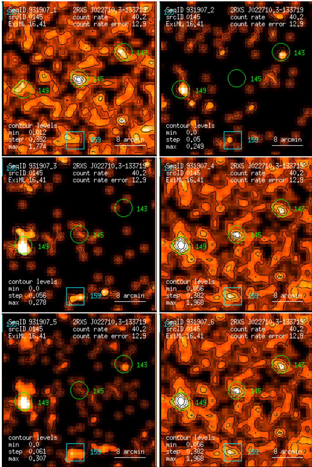
Figure 145: RASS 931907: detection 0145: band rate images, Gaussian filter: (1) PSPC channels 11 – 41, (2) 52 – 90, (3) 91 – 201, (4) 11 – 235, (5) 52 – 201, (6) 11 – 201. Broad band rates in counts/ks. Band rate contour levels in counts/ks/arcmin 2 .
