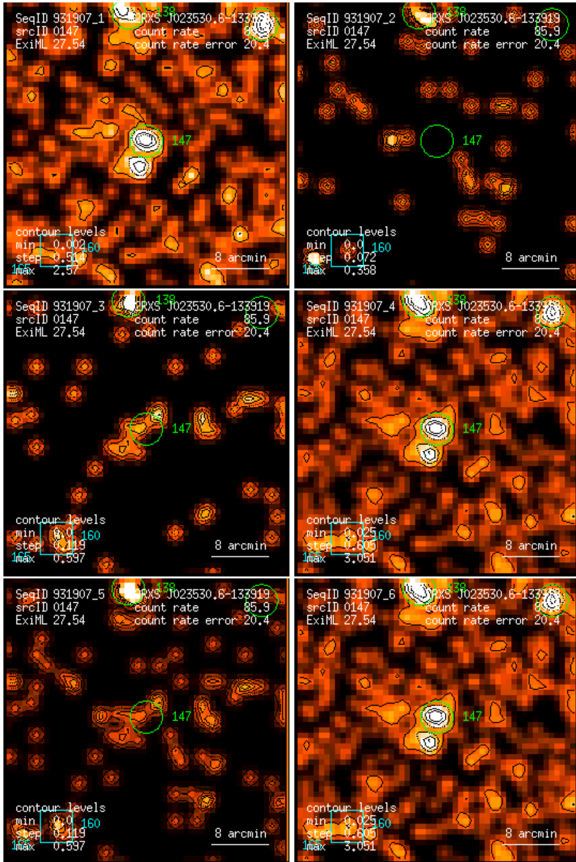
Figure 147: RASS 931907: detection 0147: band rate images, Gaussian filter: (1) PSPC channels 11 – 41, (2) 52 – 90, (3) 91 – 201, (4) 11 – 235, (5) 52 – 201, (6) 11 – 201. Broad band rates in counts/ks. Band rate contour levels in counts/ks/arcmin 2 .
