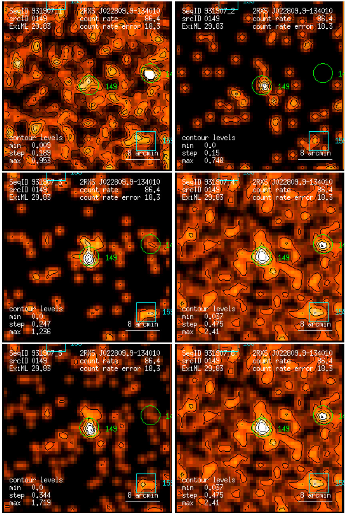
Figure 149: RASS 931907: detection 0149: band rate images, Gaussian filter: (1) PSPC channels 11 – 41, (2) 52 – 90, (3) 91 – 201, (4) 11 – 235, (5) 52 – 201, (6) 11 – 201. Broad band rates in counts/ks. Band rate contour levels in counts/ks/arcmin 2 .
