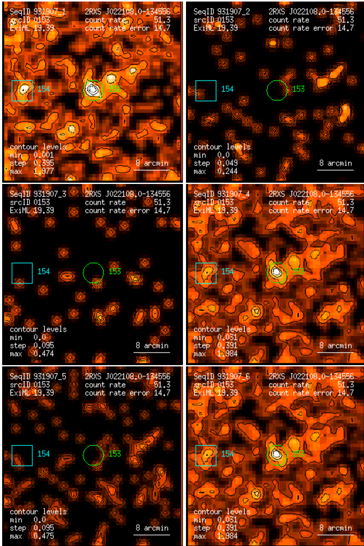
Figure 153: RASS 931907: detection 0153: band rate images, Gaussian filter: (1) PSPC channels 11 – 41, (2) 52 – 90, (3) 91 – 201, (4) 11 – 235, (5) 52 – 201, (6) 11 – 201. Broad band rates in counts/ks. Band rate contour levels in counts/ks/arcmin 2 .
