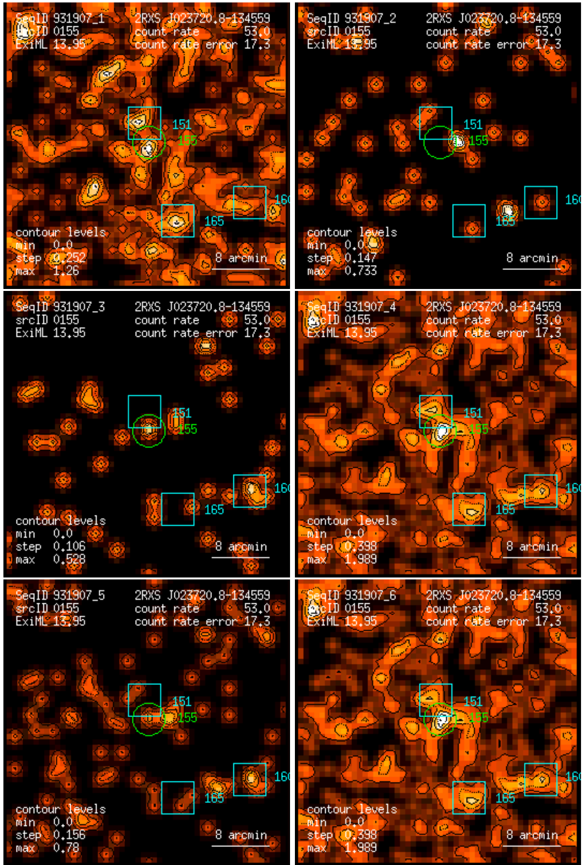
Figure 155: RASS 931907: detection 0155: band rate images, Gaussian filter: (1) PSPC channels 11 – 41, (2) 52 – 90, (3) 91 – 201, (4) 11 – 235, (5) 52 – 201, (6) 11 – 201. Broad band rates in counts/ks. Band rate contour levels in counts/ks/arcmin 2 .
