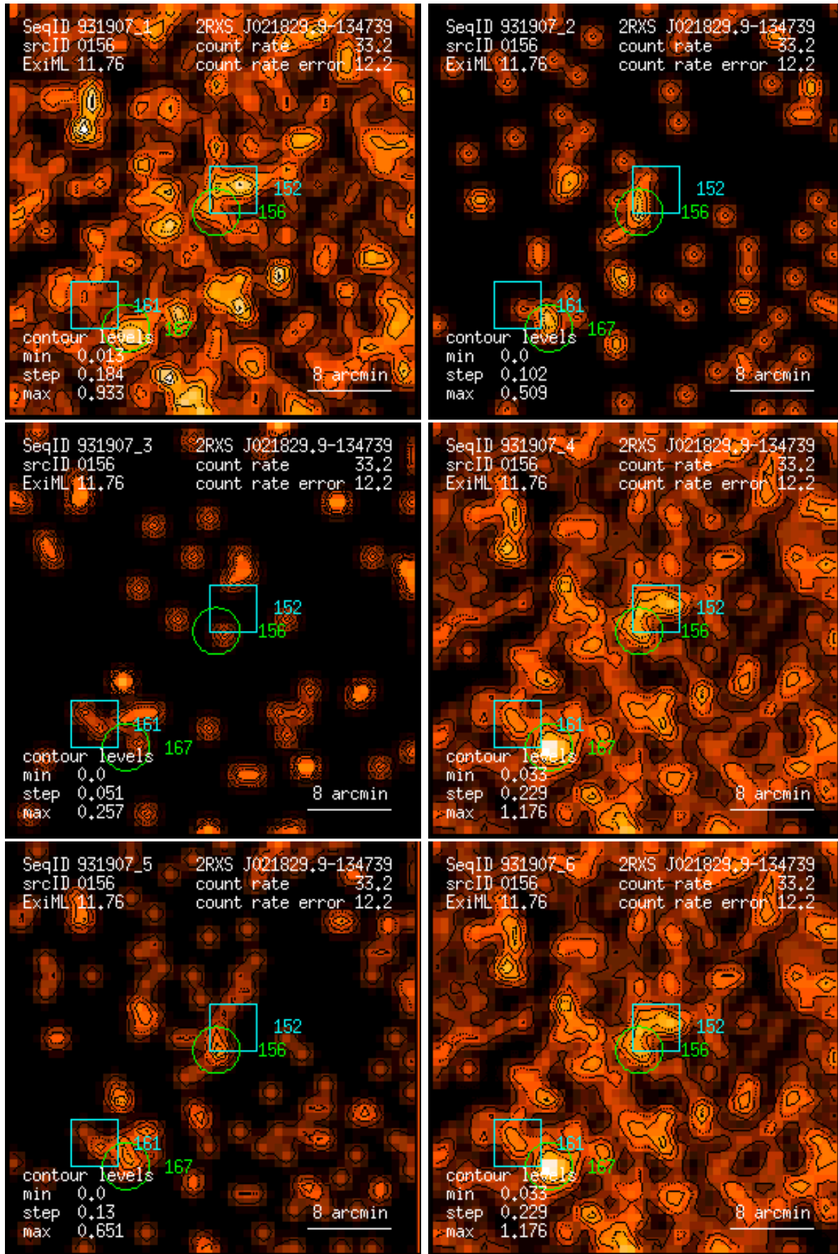
Figure 156: RASS 931907: detection 0156: band rate images, Gaussian filter: (1) PSPC channels 11 – 41, (2) 52 – 90, (3) 91 – 201, (4) 11 – 235, (5) 52 – 201, (6) 11 – 201. Broad band rates in counts/ks. Band rate contour levels in counts/ks/arcmin 2 .
