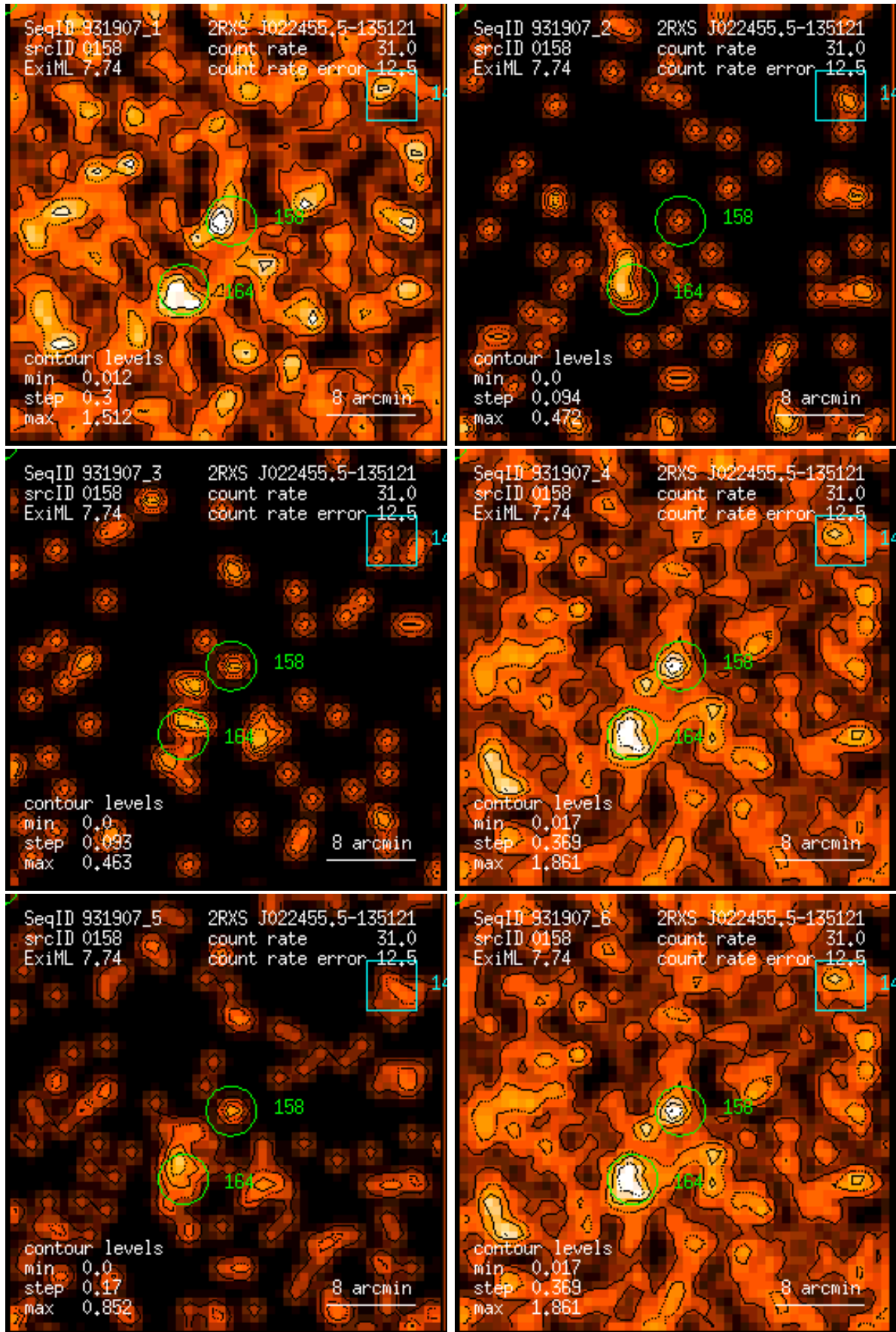
Figure 158: RASS 931907: detection 0158: band rate images, Gaussian filter: (1) PSPC channels 11 – 41, (2) 52 – 90, (3) 91 – 201, (4) 11 – 235, (5) 52 – 201, (6) 11 – 201. Broad band rates in counts/ks. Band rate contour levels in counts/ks/arcmin 2 .
