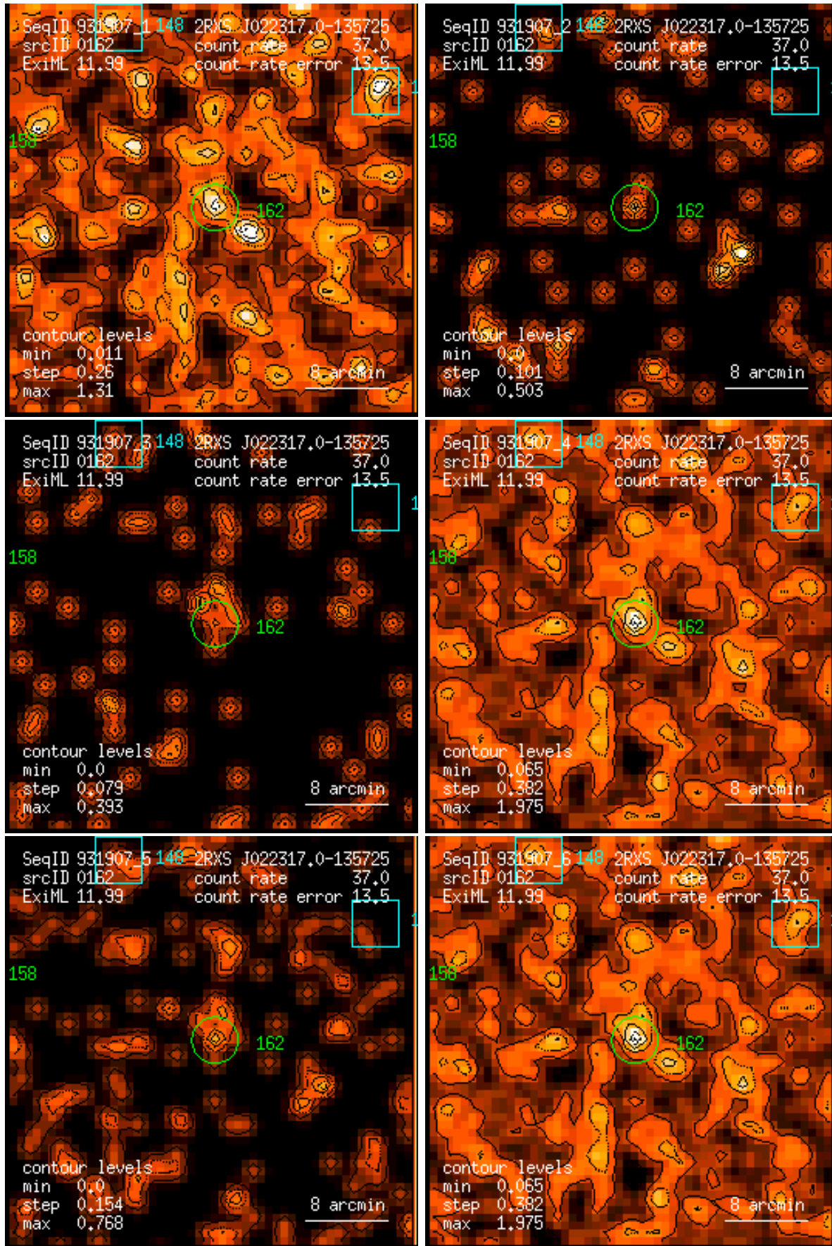
Figure 162: RASS 931907: detection 0162: band rate images, Gaussian filter: (1) PSPC channels 11 – 41, (2) 52 – 90, (3) 91 – 201, (4) 11 – 235, (5) 52 – 201, (6) 11 – 201. Broad band rates in counts/ks. Band rate contour levels in counts/ks/arcmin 2 .
