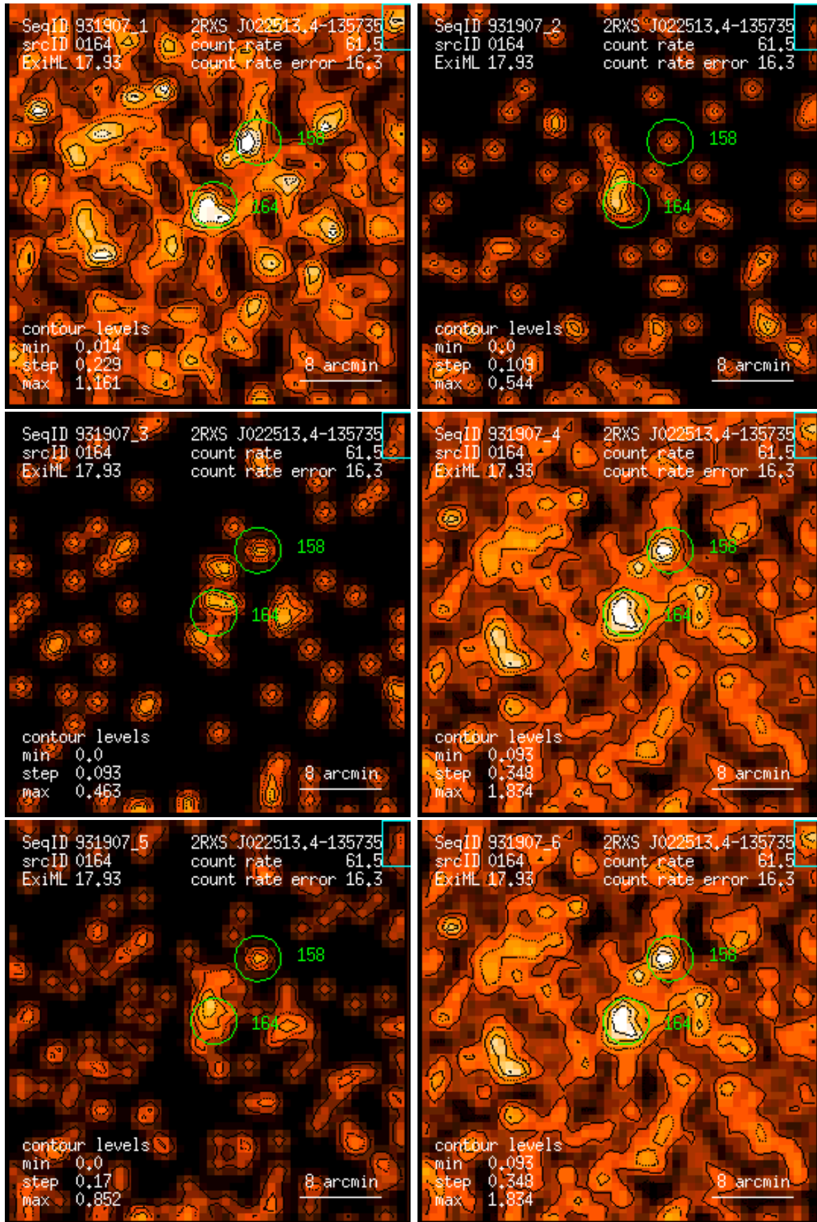
Figure 164: RASS 931907: detection 0164: band rate images, Gaussian filter: (1) PSPC channels 11 – 41, (2) 52 – 90, (3) 91 – 201, (4) 11 – 235, (5) 52 – 201, (6) 11 – 201. Broad band rates in counts/ks. Band rate contour levels in counts/ks/arcmin 2 .
