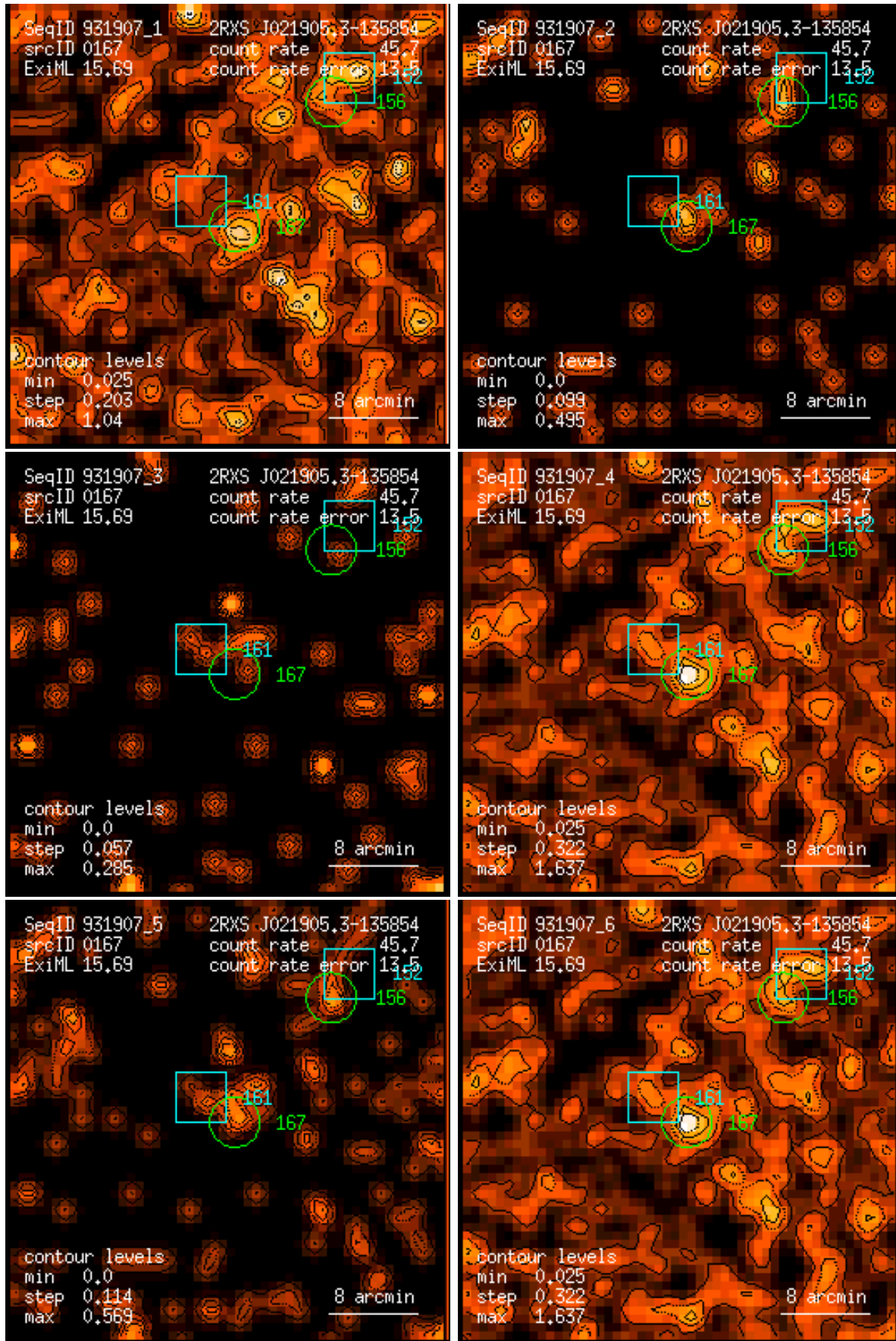
Figure 167: RASS 931907: detection 0167: band rate images, Gaussian filter: (1) PSPC channels 11 – 41, (2) 52 – 90, (3) 91 – 201, (4) 11 – 235, (5) 52 – 201, (6) 11 – 201. Broad band rates in counts/ks. Band rate contour levels in counts/ks/arcmin 2 .
