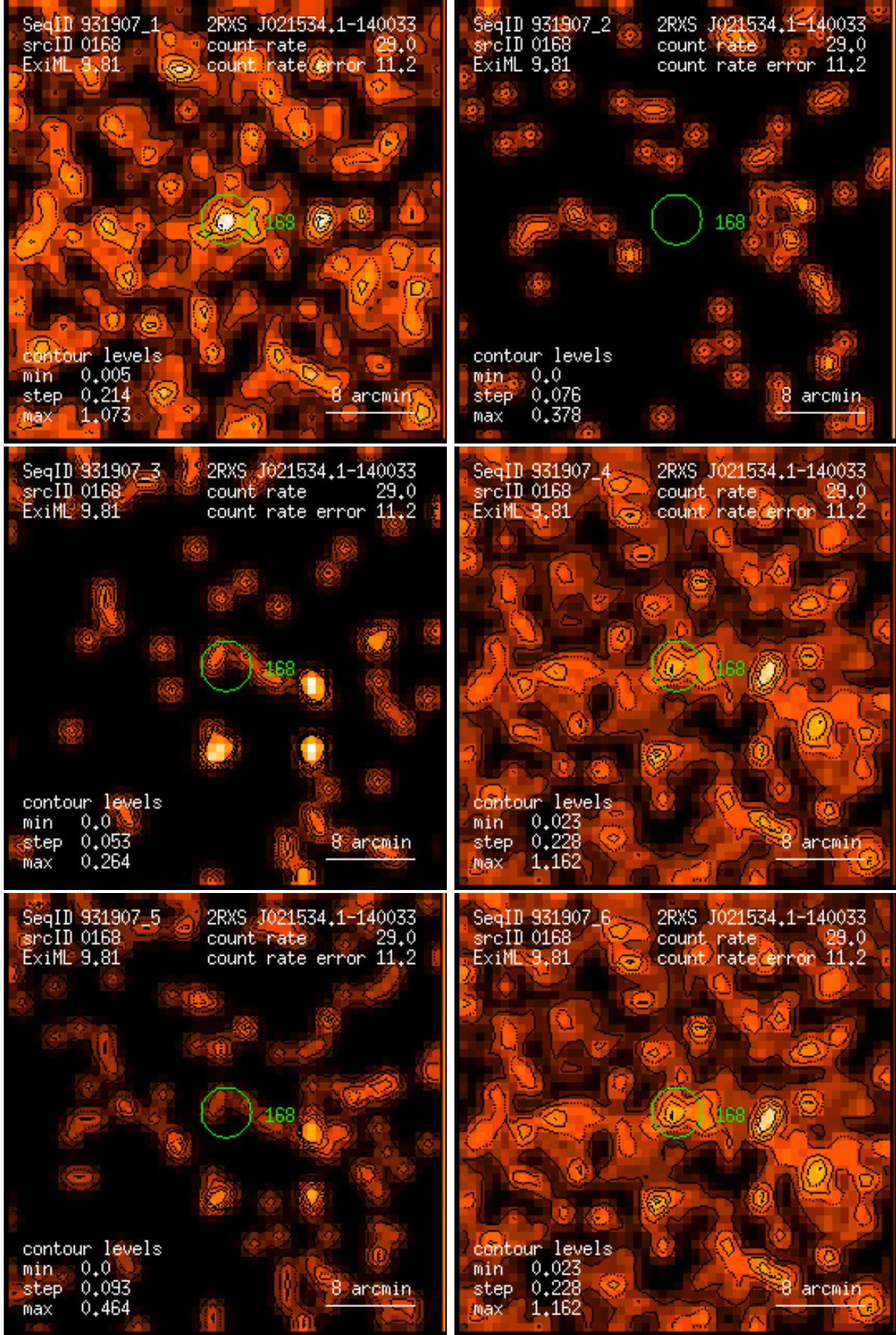
Figure 168: RASS 931907: detection 0168: band rate images, Gaussian filter: (1) PSPC channels 11 – 41, (2) 52 – 90, (3) 91 – 201, (4) 11 – 235, (5) 52 – 201, (6) 11 – 201. Broad band rates in counts/ks. Band rate contour levels in counts/ks/arcmin 2 .
