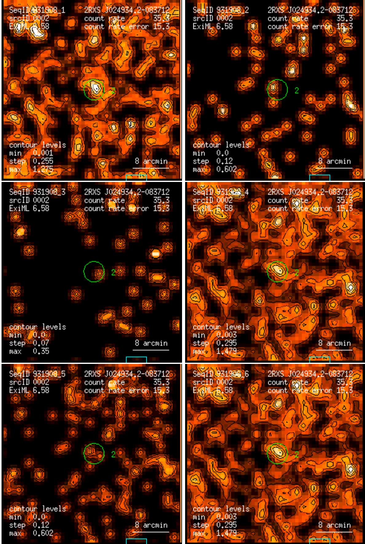
Figure 2: RASS 931908: detection 0002: band rate images, Gaussian filter: (1) PSPC channels 11 – 41, (2) 52 – 90, (3) 91 – 201, (4) 11 – 235, (5) 52 – 201, (6) 11 – 201. Broad band rates in counts/ks. Band rate contour levels in counts/ks/arcmin 2 .
