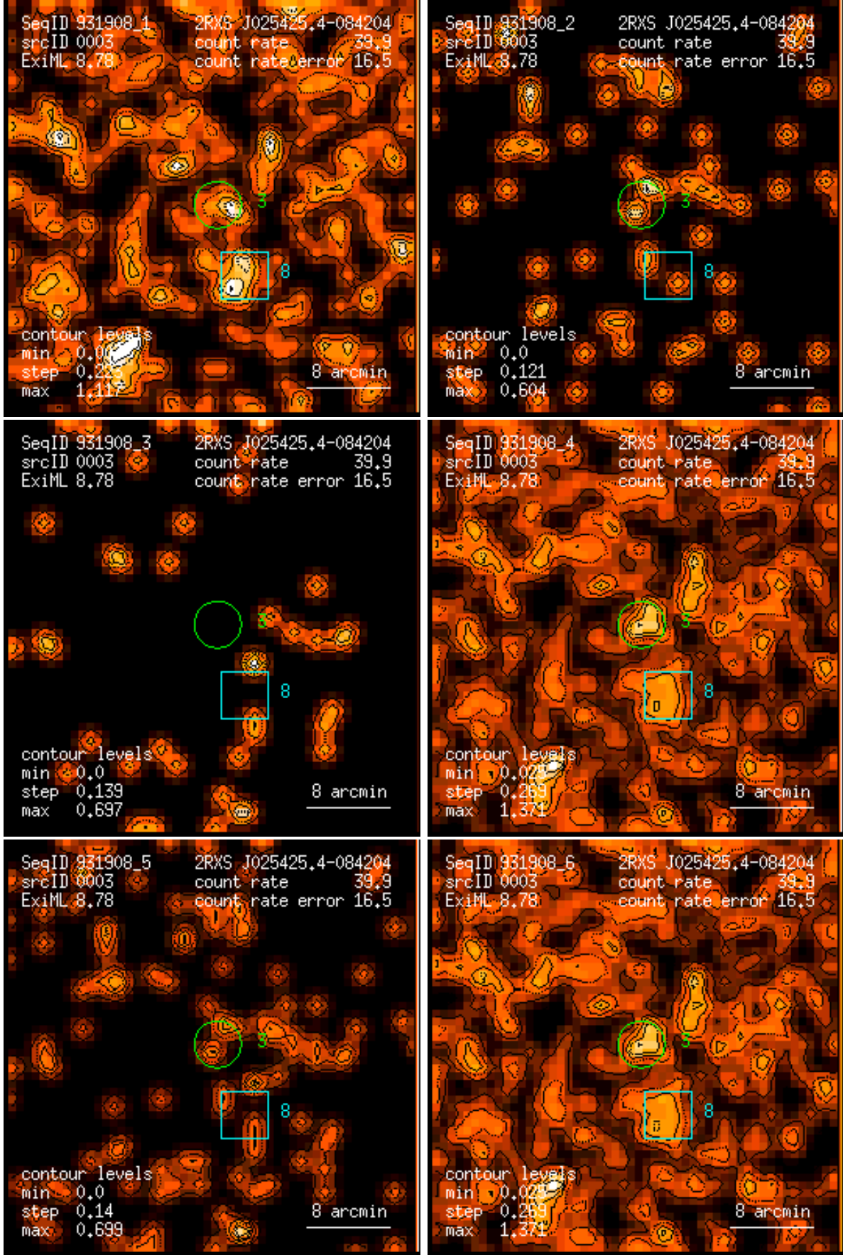
Figure 3: RASS 931908: detection 0003: band rate images, Gaussian filter: (1) PSPC channels 11 – 41, (2) 52 – 90, (3) 91 – 201, (4) 11 – 235, (5) 52 – 201, (6) 11 – 201. Broad band rates in counts/ks. Band rate contour levels in counts/ks/arcmin 2 .
