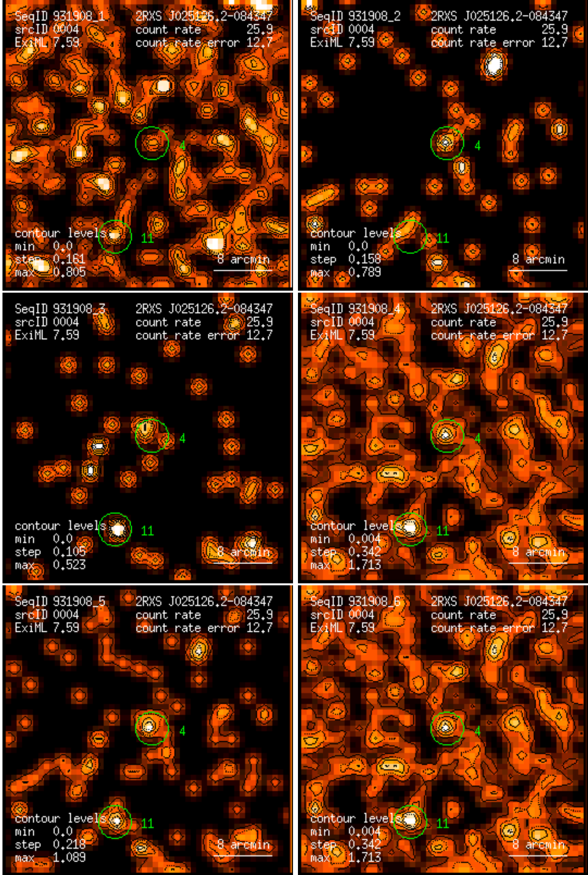
Figure 4: RASS 931908: detection 0004: band rate images, Gaussian filter: (1) PSPC channels 11 – 41, (2) 52 – 90, (3) 91 – 201, (4) 11 – 235, (5) 52 – 201, (6) 11 – 201. Broad band rates in counts/ks. Band rate contour levels in counts/ks/arcmin 2 .
