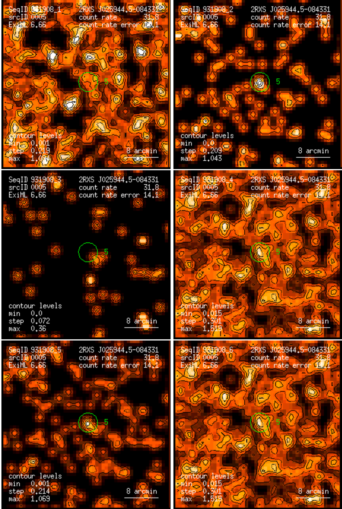
Figure 5: RASS 931908: detection 0005: band rate images, Gaussian filter: (1) PSPC channels 11 – 41, (2) 52 – 90, (3) 91 – 201, (4) 11 – 235, (5) 52 – 201, (6) 11 – 201. Broad band rates in counts/ks. Band rate contour levels in counts/ks/arcmin 2 .
