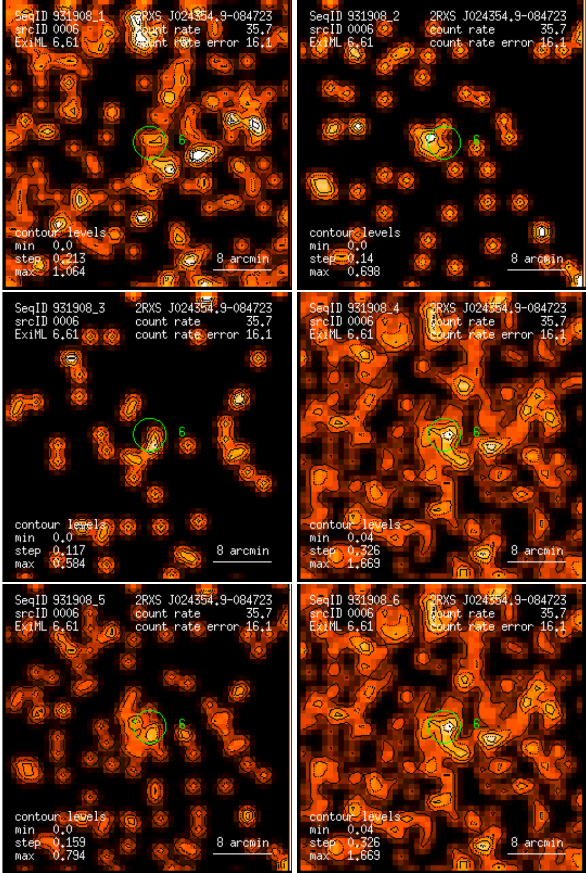
Figure 6: RASS 931908: detection 0006: band rate images, Gaussian filter: (1) PSPC channels 11 – 41, (2) 52 – 90, (3) 91 – 201, (4) 11 – 235, (5) 52 – 201, (6) 11 – 201. Broad band rates in counts/ks. Band rate contour levels in counts/ks/arcmin 2 .
