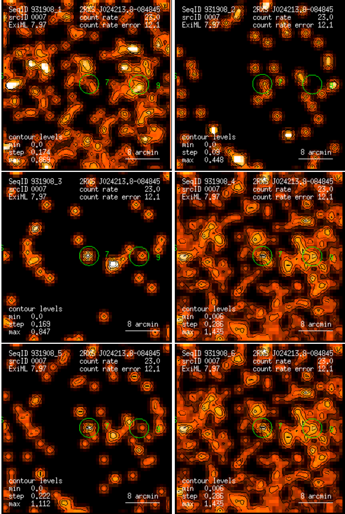
Figure 7: RASS 931908: detection 0007: band rate images, Gaussian filter: (1) PSPC channels 11 – 41, (2) 52 – 90, (3) 91 – 201, (4) 11 – 235, (5) 52 – 201, (6) 11 – 201. Broad band rates in counts/ks. Band rate contour levels in counts/ks/arcmin 2 .
